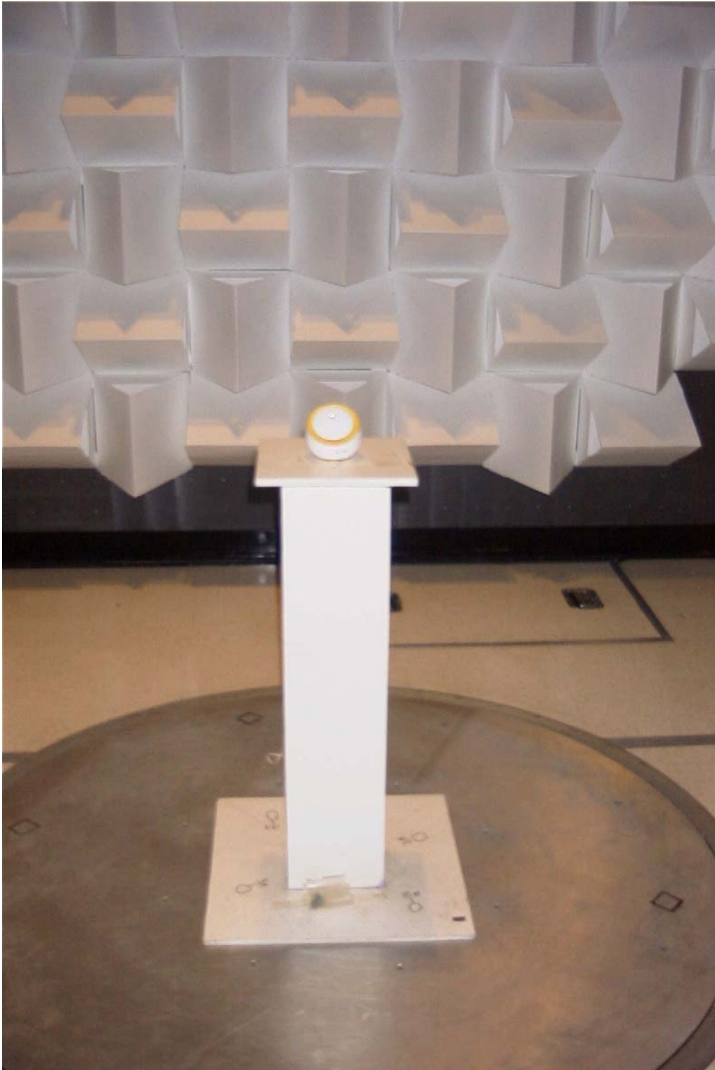
RADIATED TEST SET UP (BASE) – MODEL SCD588:
