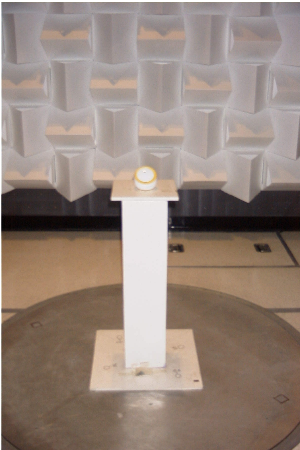
RADIATED TEST SET UP (BASE) – MODEL SCD587:
