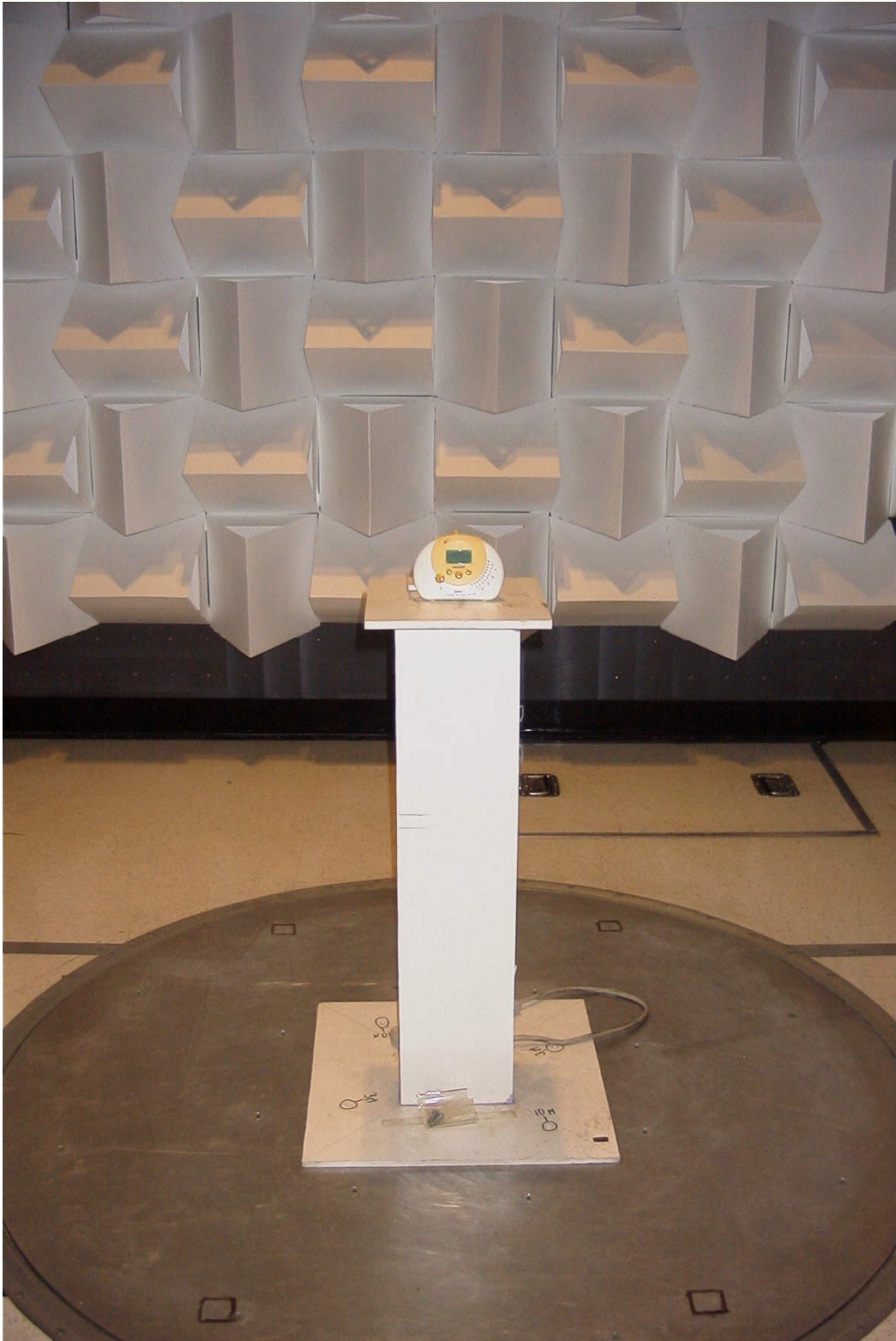
RADIATED TEST SET UP (BASE) MODEL SCD386:
