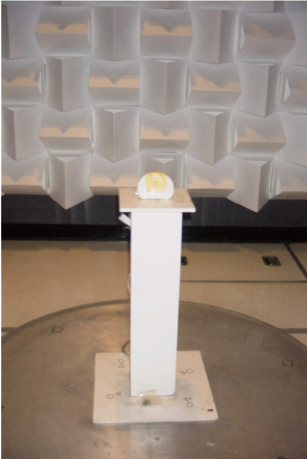
RADIATED TEST SET UP (BASE) MODEL SCD384:
