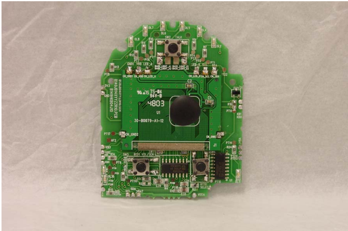
TOP VIEW 1
