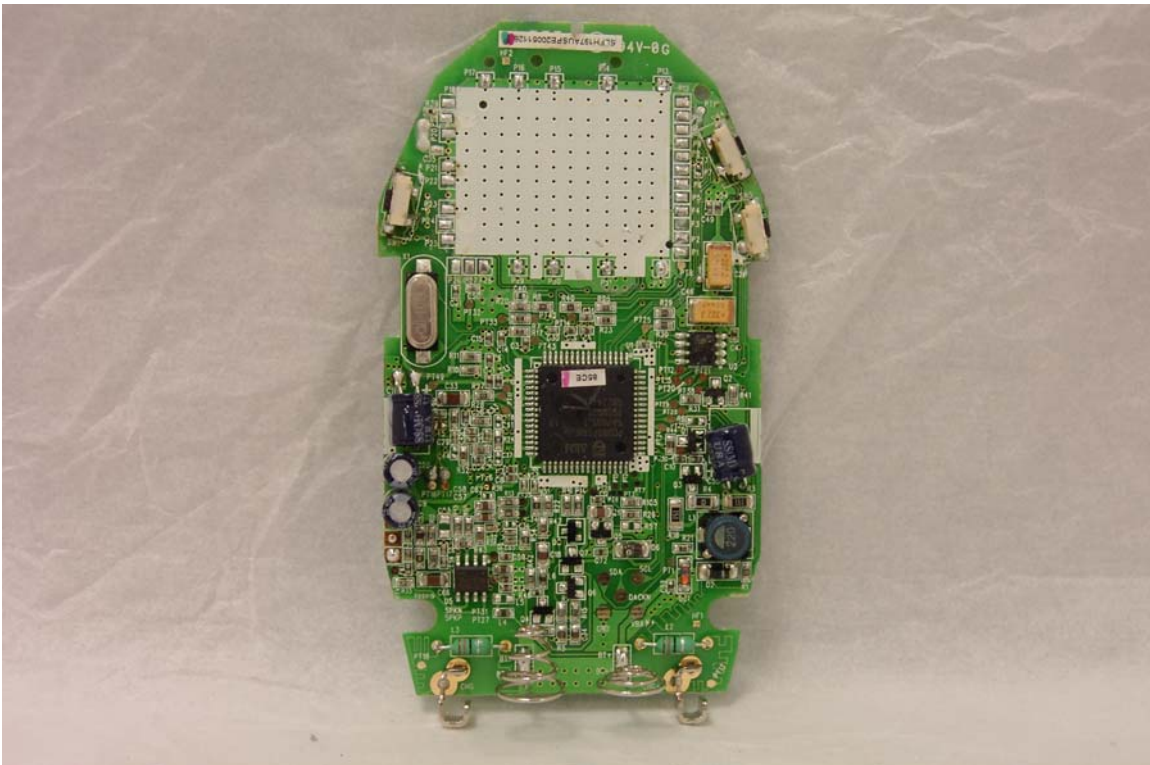
TOP VIEW 2
