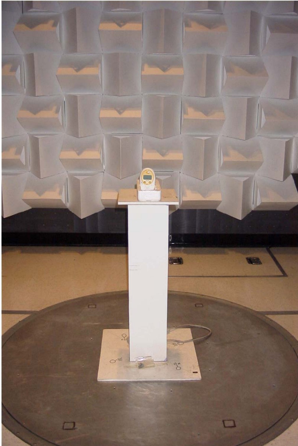
RADIATED TEST SET UP (HANDSET) – MODEL SCD386R:
