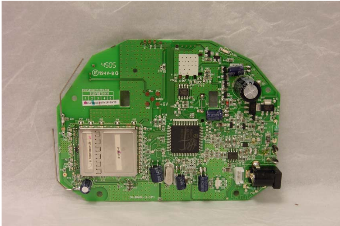
TOP VIEW 1
