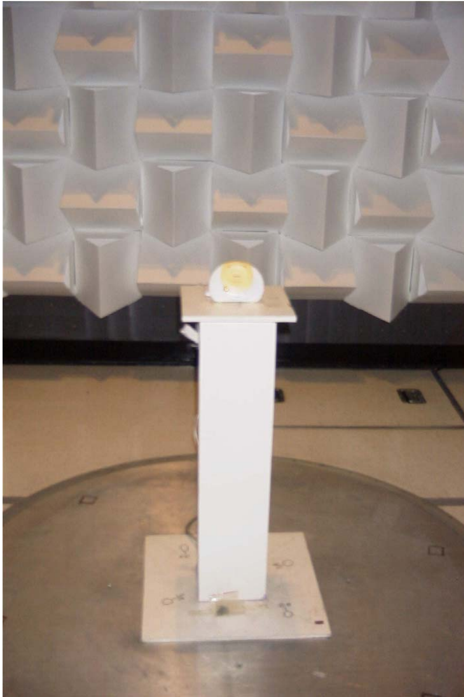
RADIATED TEST SET UP (BASE) MODEL SCD384:
