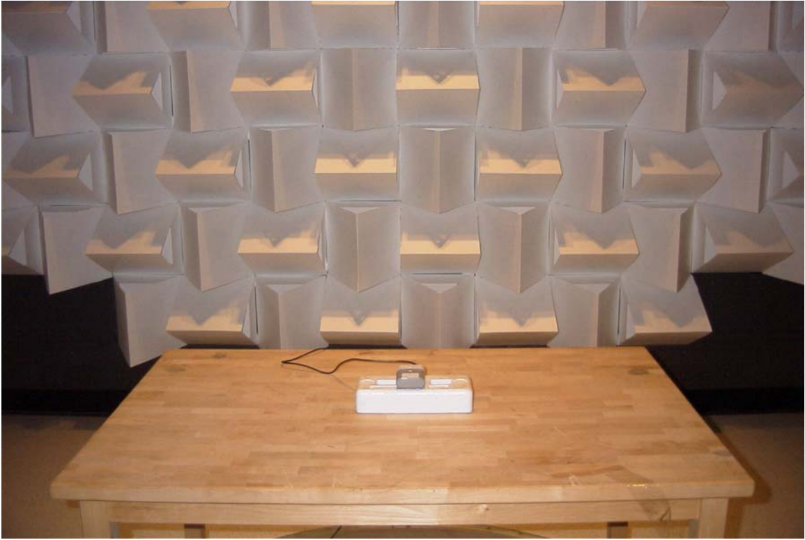
RADIATED EMISSIONS TEST SET UP
