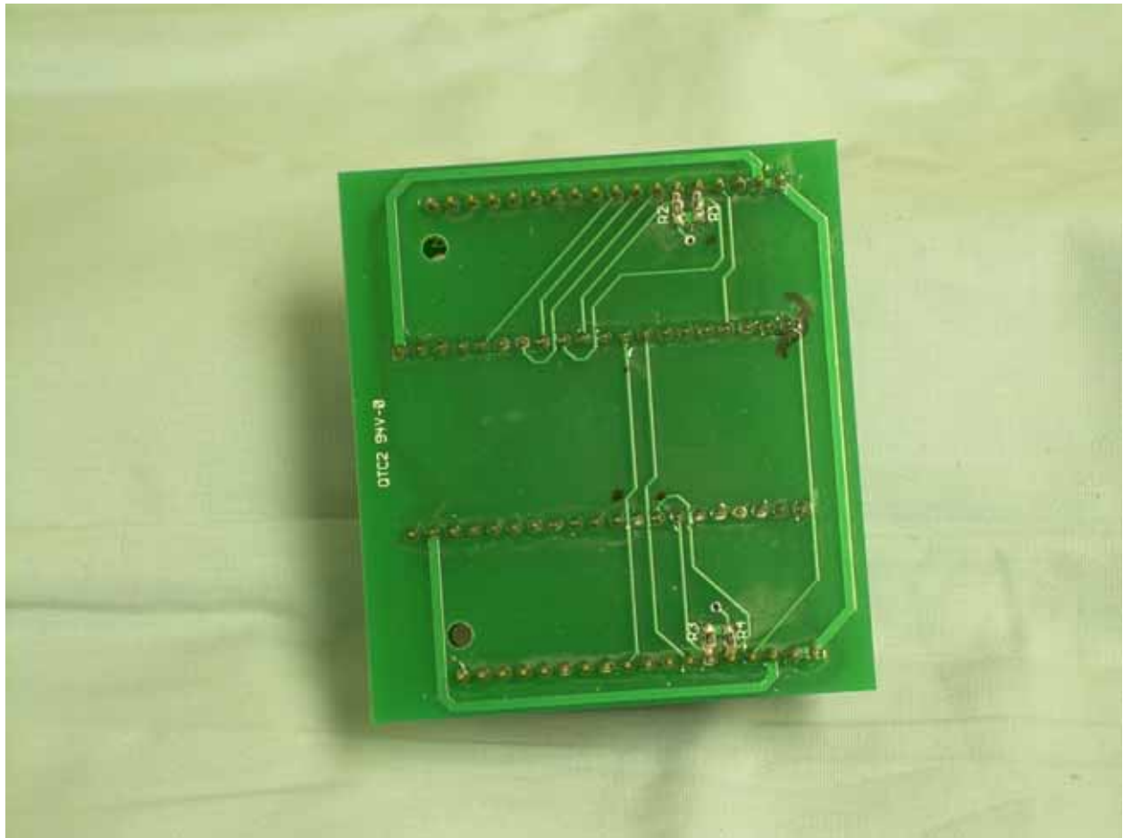
Photograph 17 – View of the Bottom Side of the Header PCB
