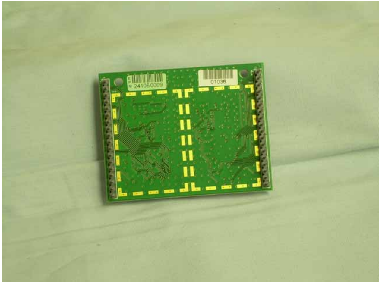
Photograph 13 – View of the Trace Side of the EUT RF PCB
