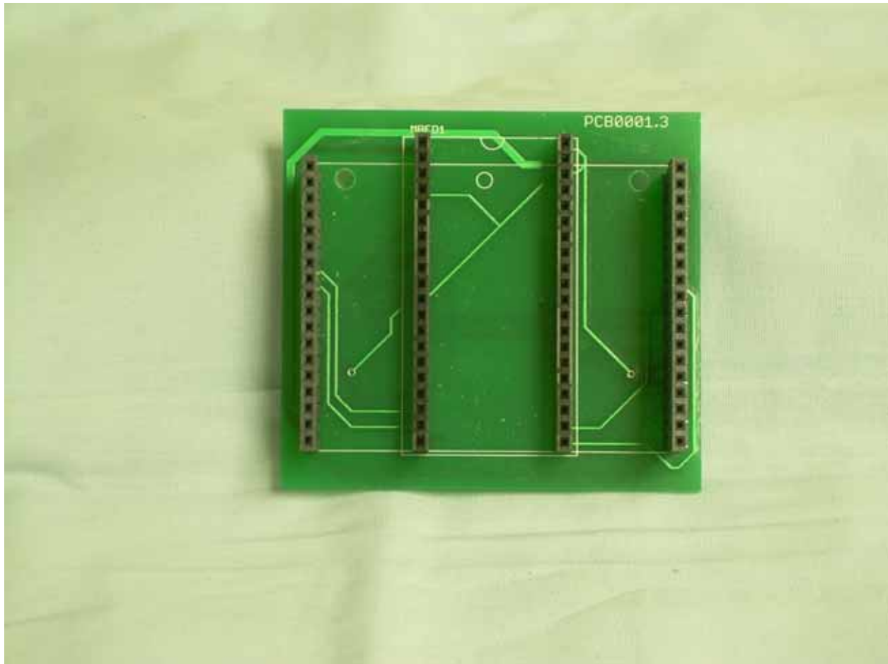
Photograph 16 – View of the Top Side of the Header PCB
