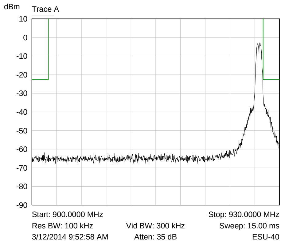
Trace A operating band
