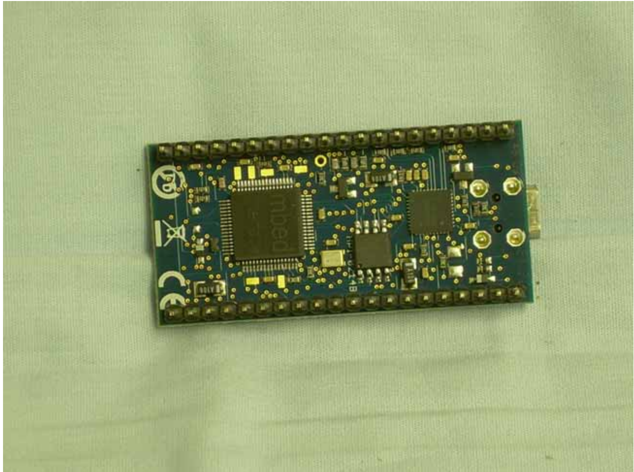
Photograph 15 – View of the Bottom Side of the System Interface PCB
