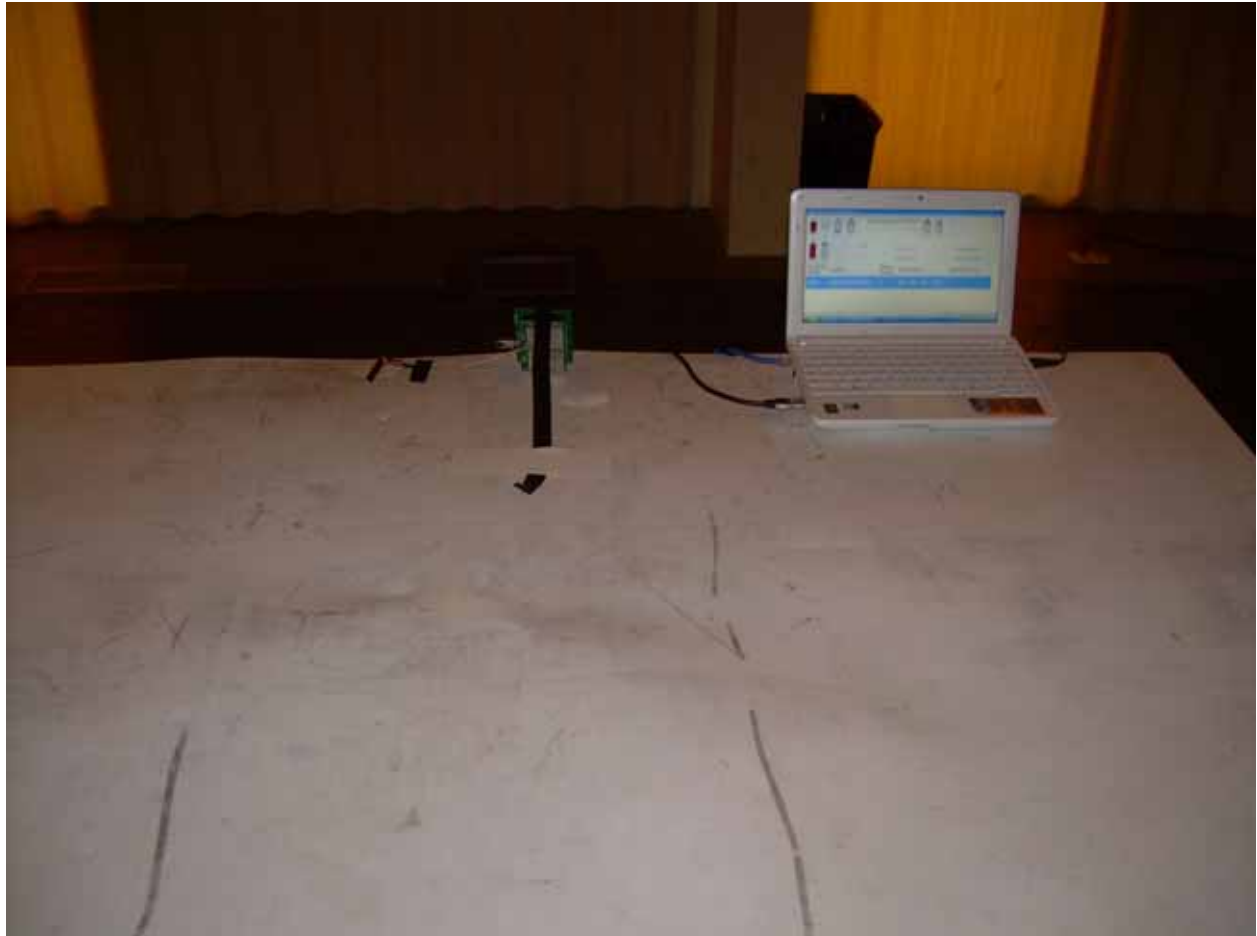
Photograph 5 – Front View Radiated Emission – On Edge Configuration
