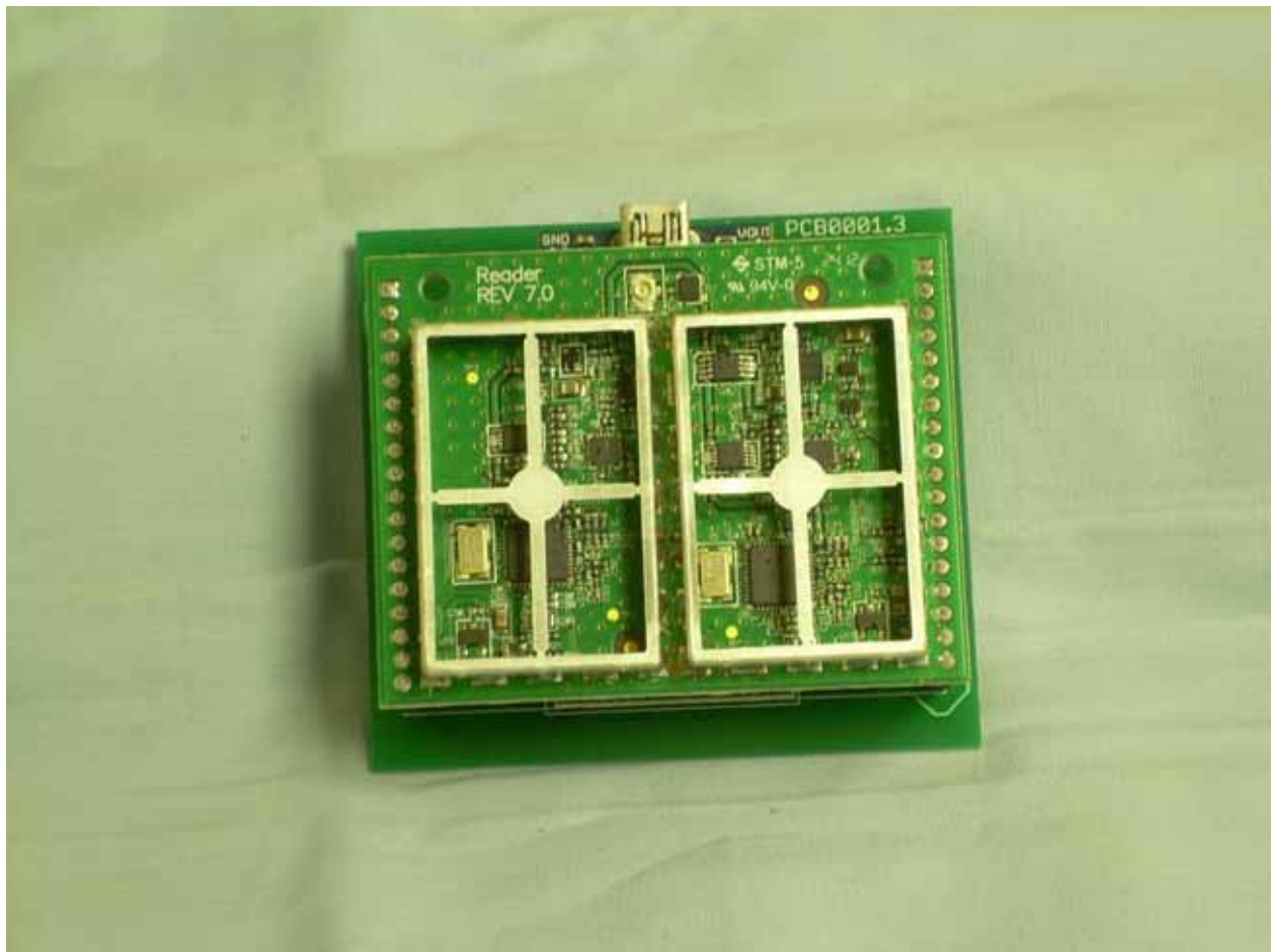
Photograph 12 – View of the Component Side of the EUT RF PCB with RF Shield Tops Removed
