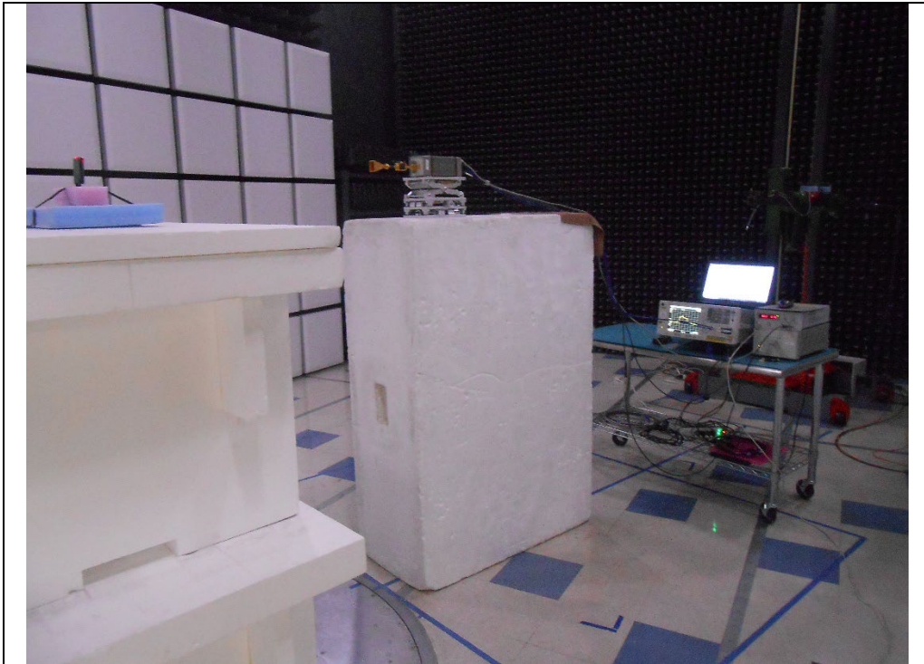
RF Radiated_ 50 – 75 GHz
