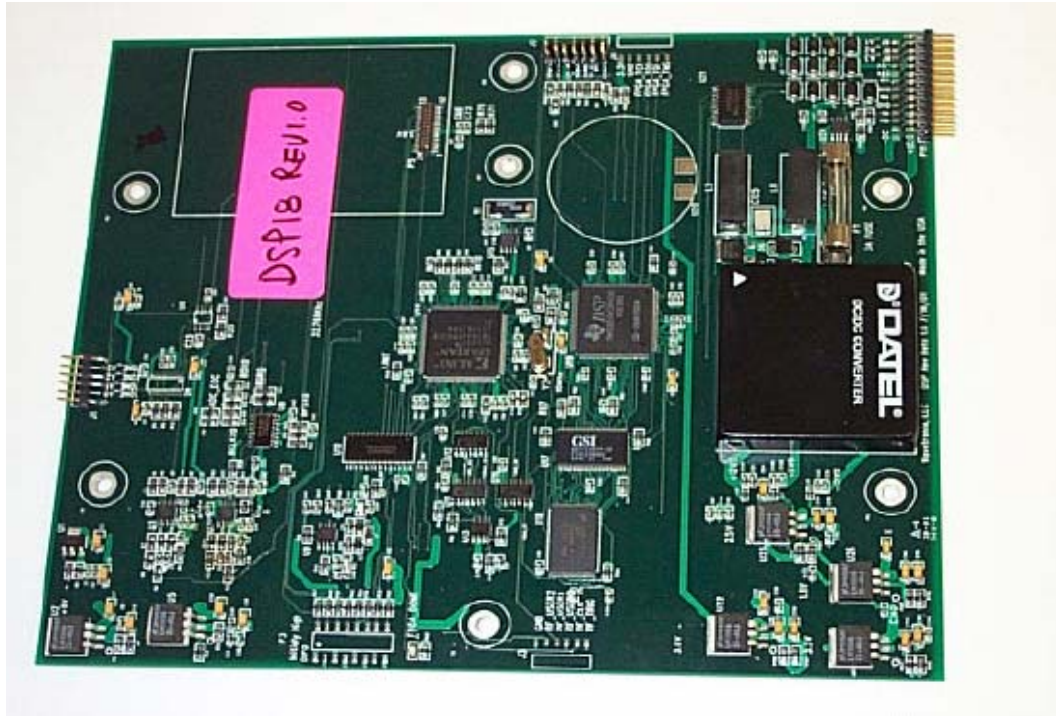
Main Board
