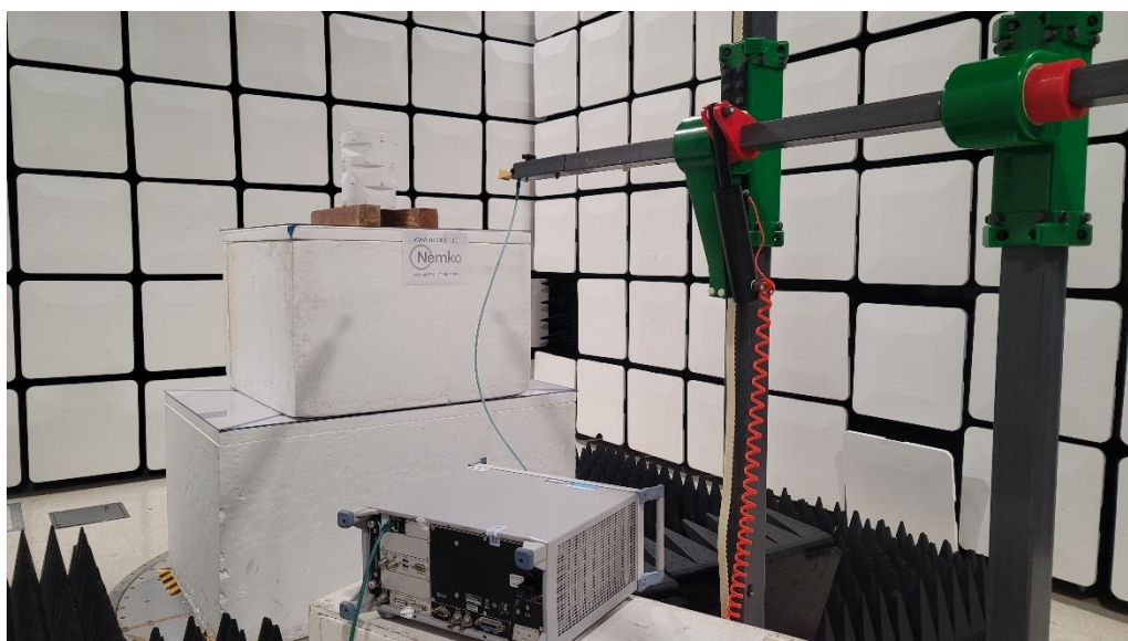
Figure 10 - Radiated emissions above 1 GHz (40 – 50 GHz), front view
