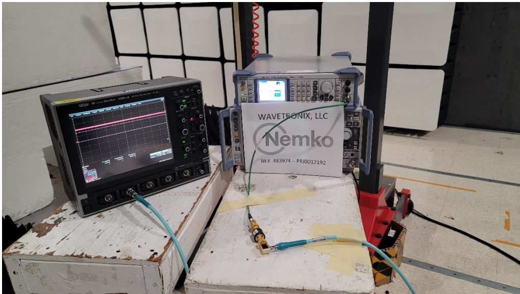
Figure 21- E.I.R.P. Conducted measurement
