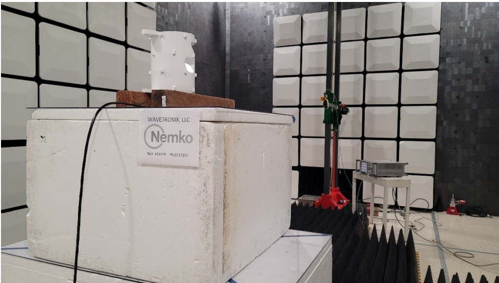
Figure 9 - Radiated emissions above 1 GHz (26 – 40 GHz), rear view
