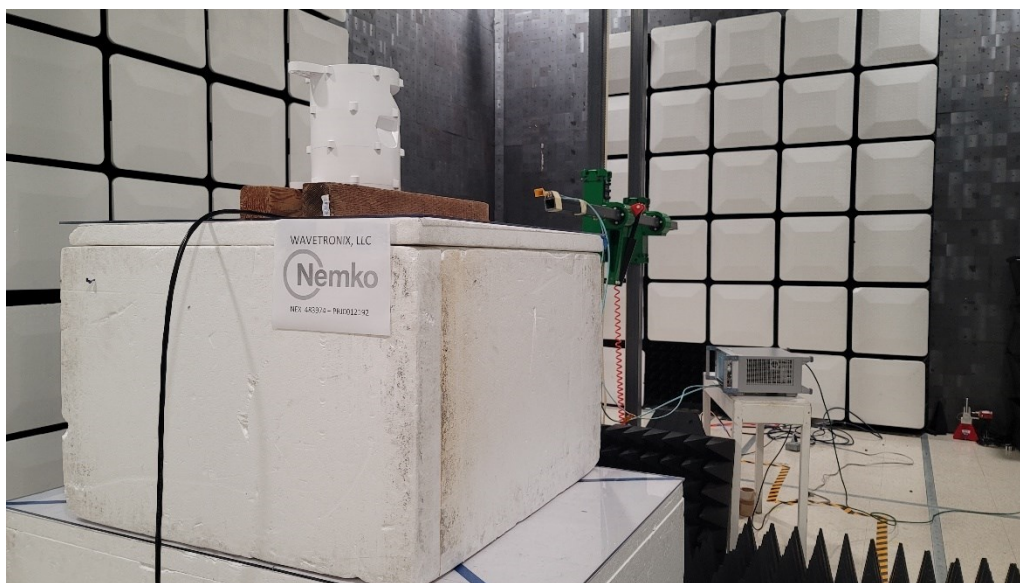
Figure 13 - Radiated emissions above 1 GHz (50 – 75 GHz), rear view
