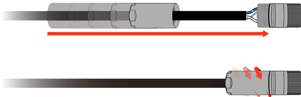
Figure 17. Tighten connector
