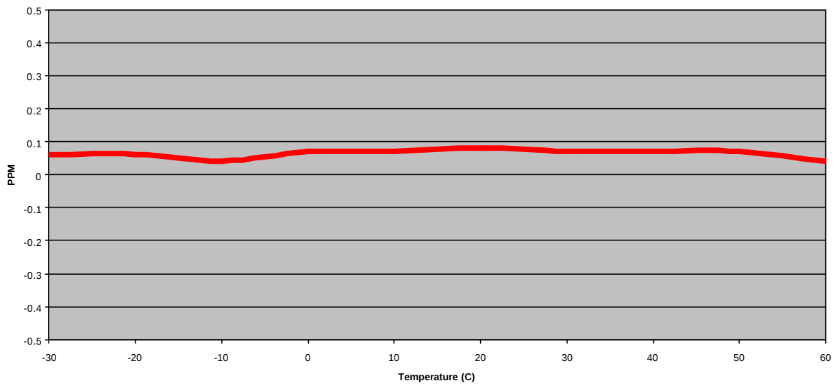
Temperature Frequency Stability
