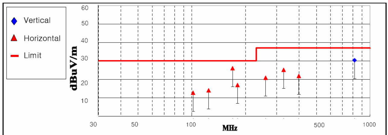
Fig 5. Graph of Radiated emission – Play Mode
