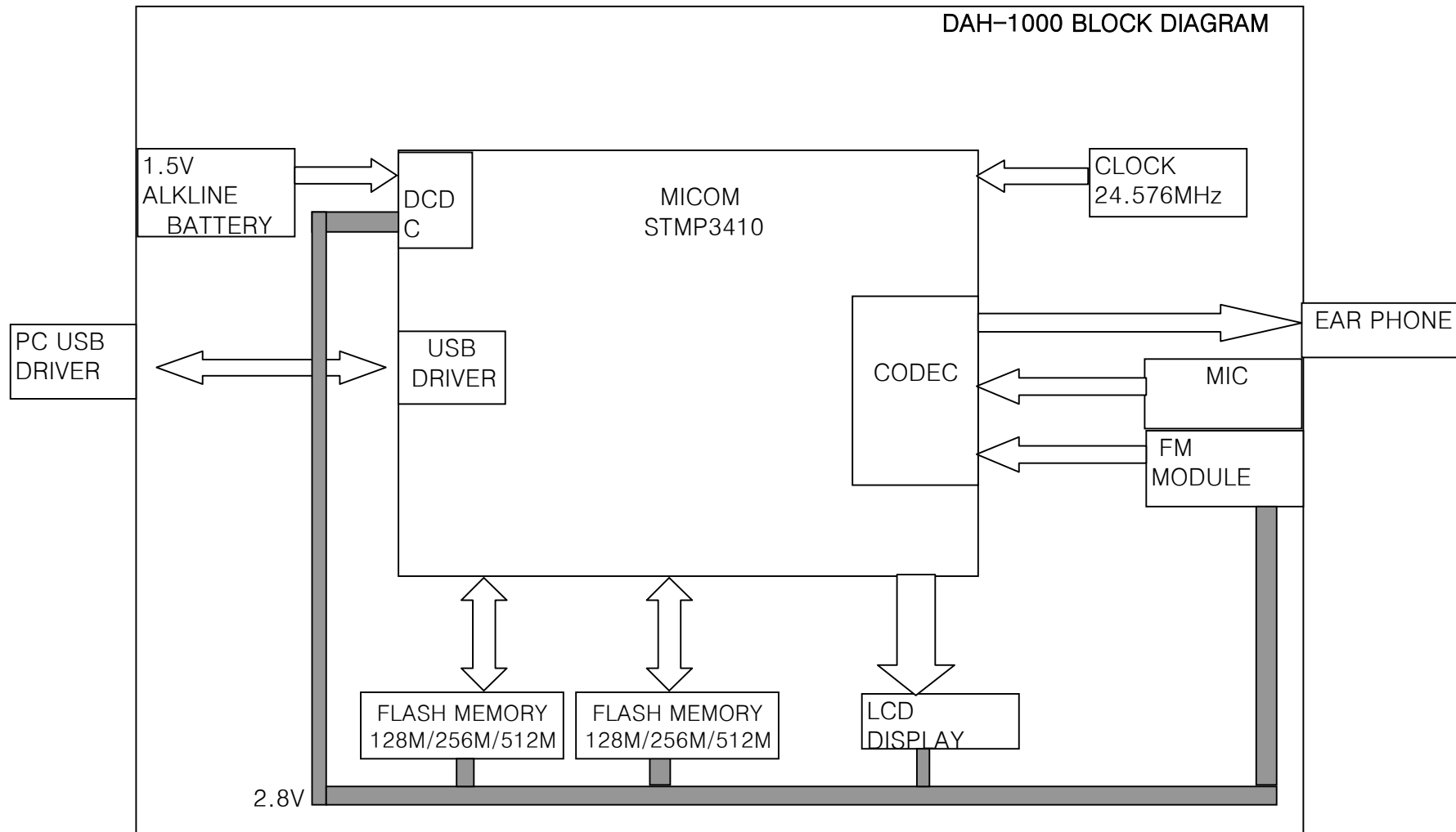
DAH-1000 BLOCK DIAGRAM
