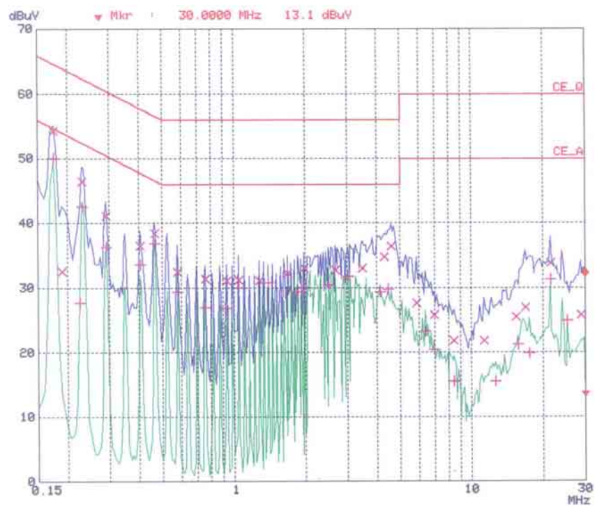
< Neutral line >
