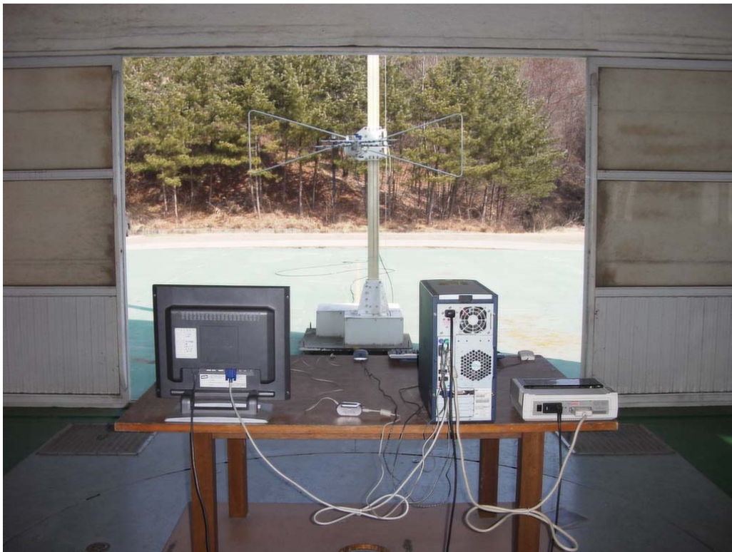
Radiated Emissions (File up/download mode) - Rear View
