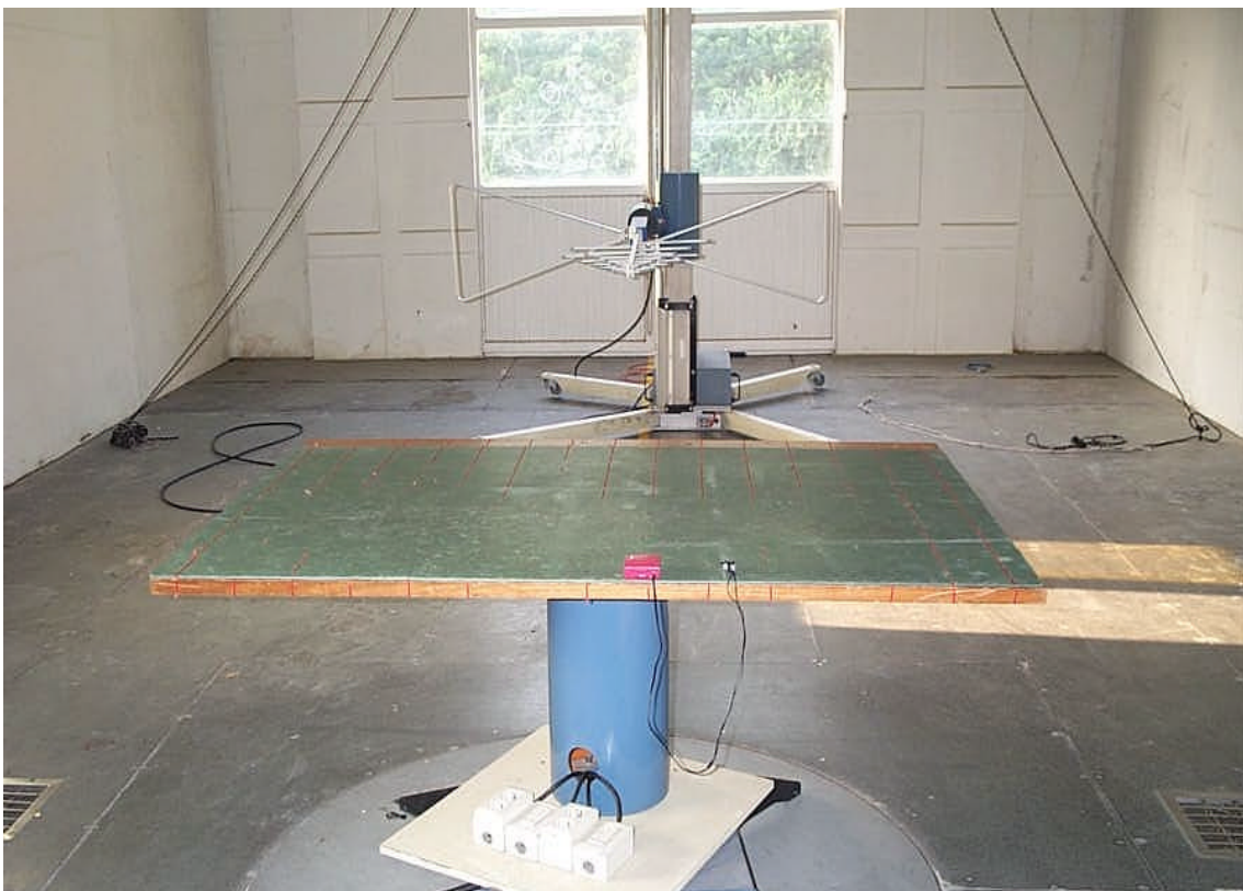
Radiated Emission 30MHz ~ 1000MHz ( Play Mode )
