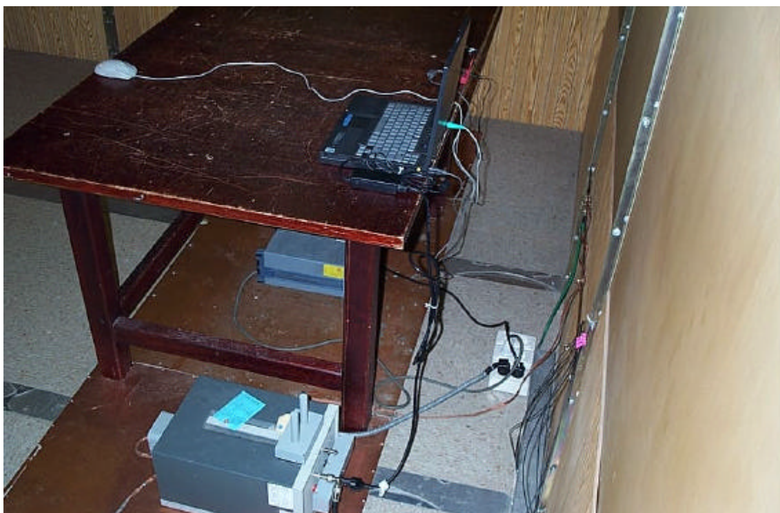
Conducted Emission 450kHz ~ 30MHz ( File Download Mode )
