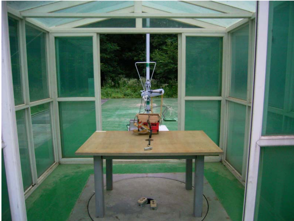
Radiated Emissions(charging /Playback mode)- Front View
