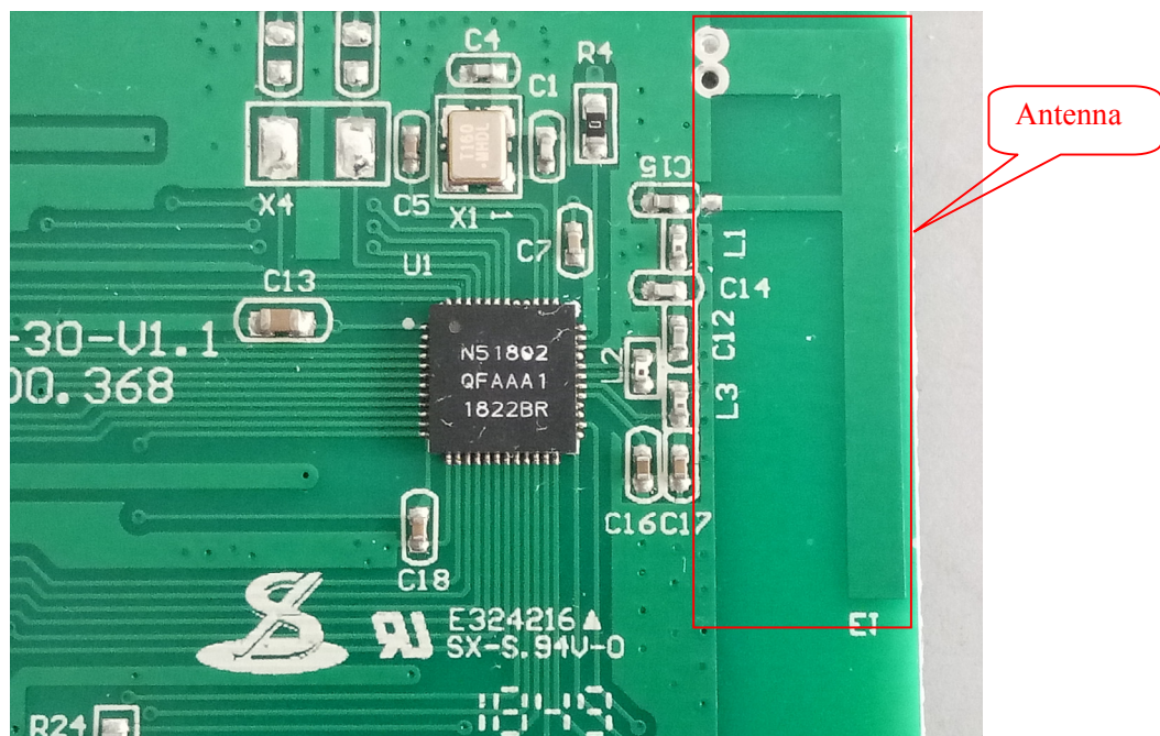
EUT – PCB chip View-1
