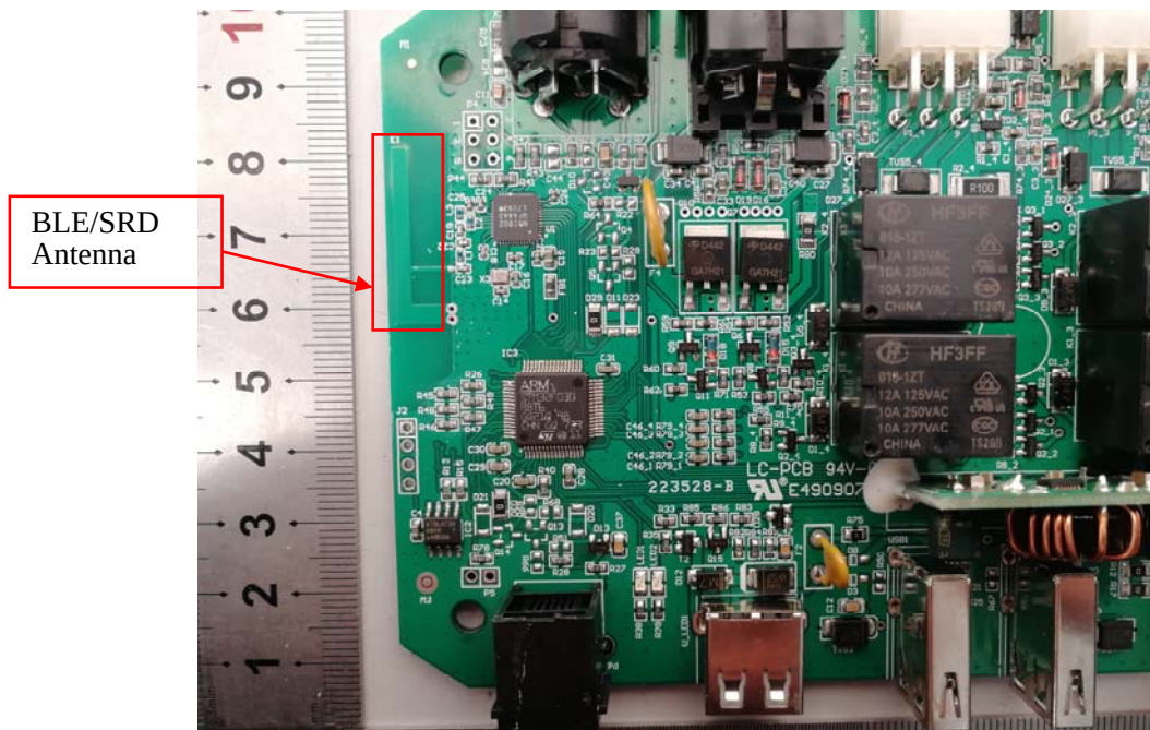
EUT – PCB chip View
