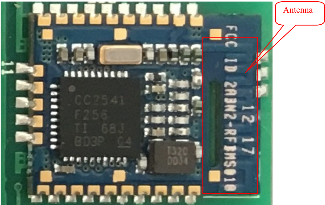
EUT – Module View
