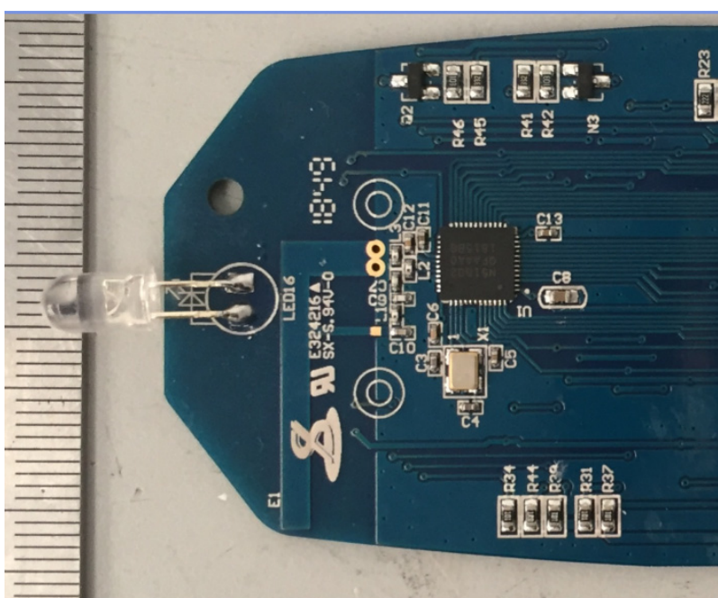
EUT – PCB Top Chip View
