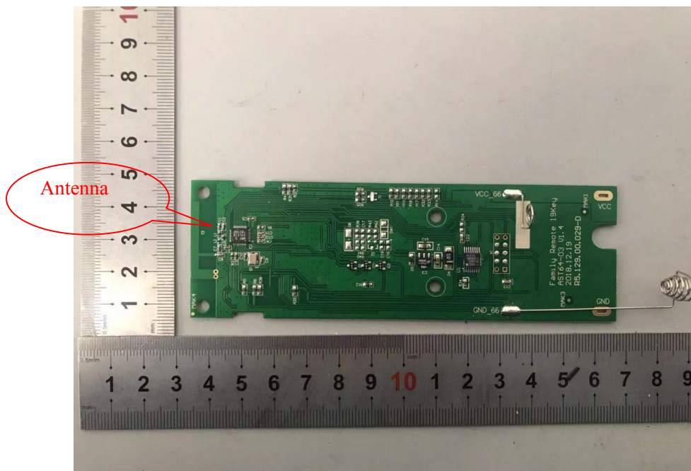
EUT – PCB IC Chip View
