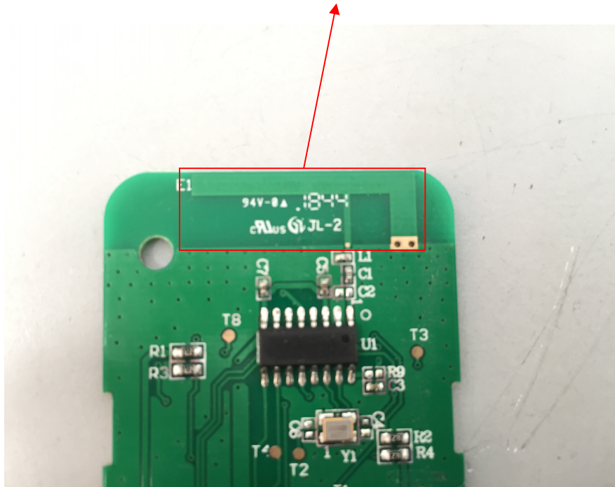
EUT – PCB Antenna View
