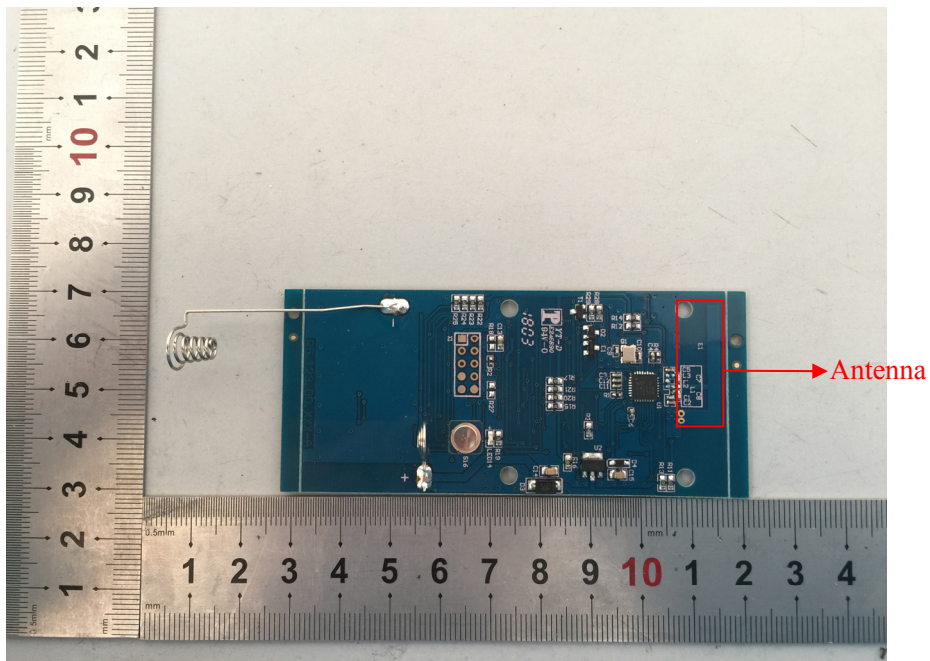
EUT – PCB Top View
