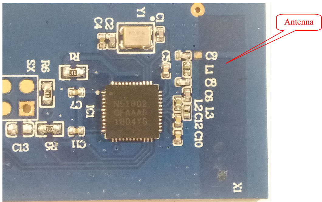
EUT – PCB Bottom View
