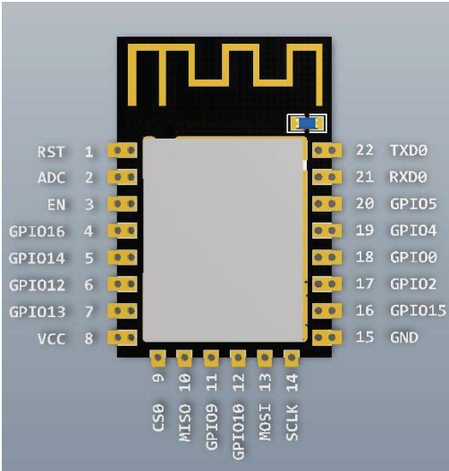
Figure 2 pinout
