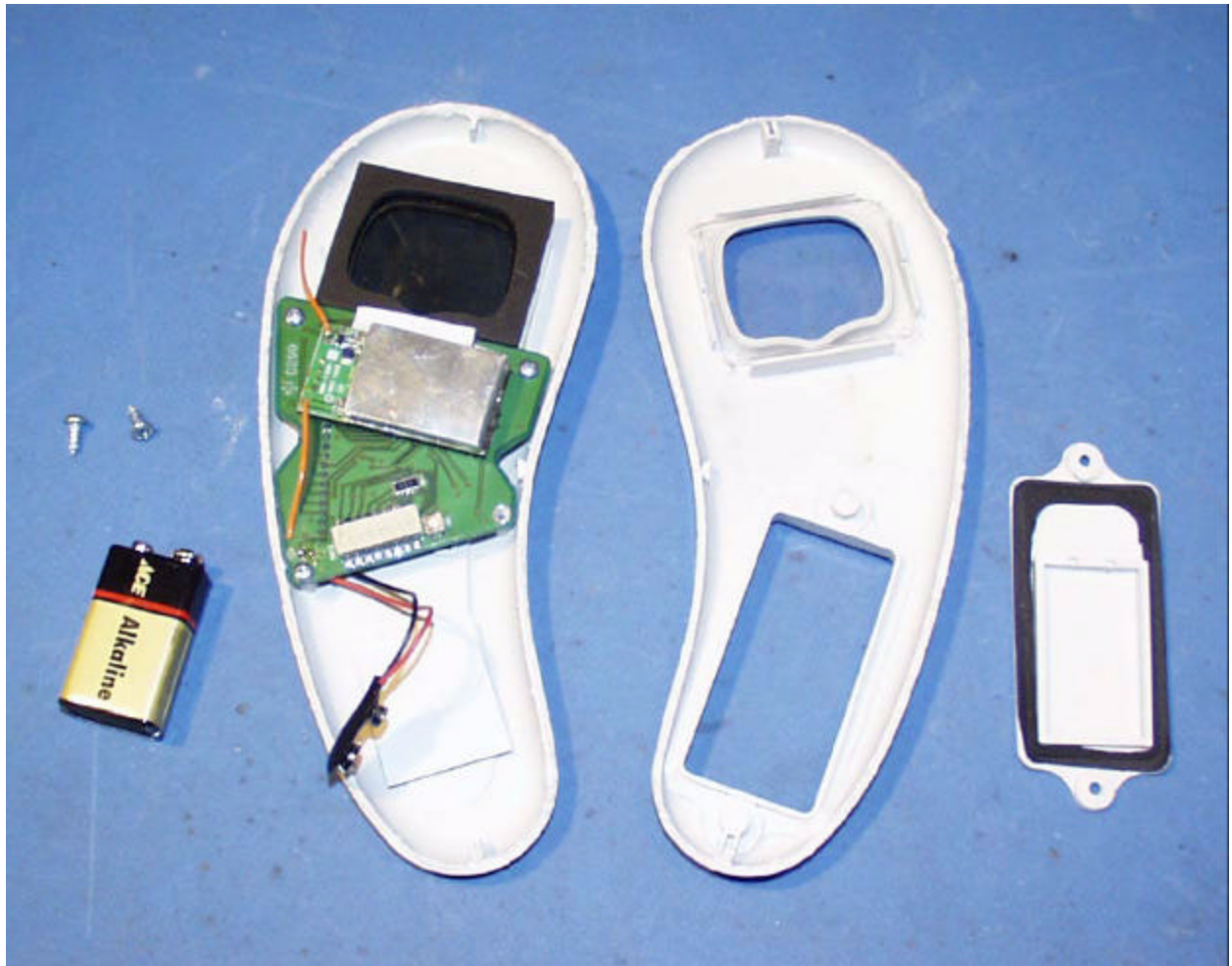
Inside Rear Cover
