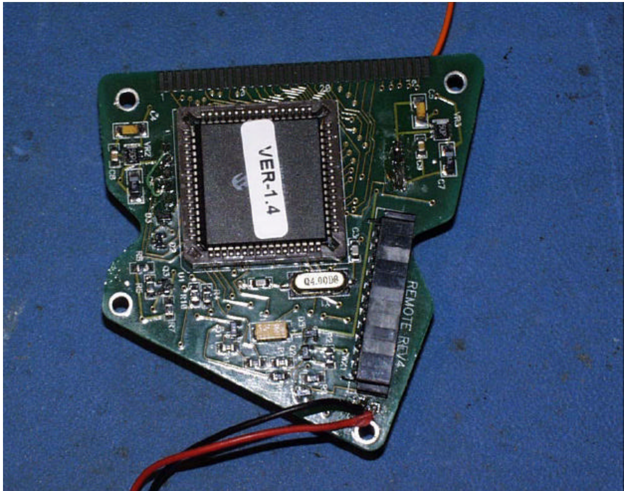
Transceiver and Control Board, Foil Side
