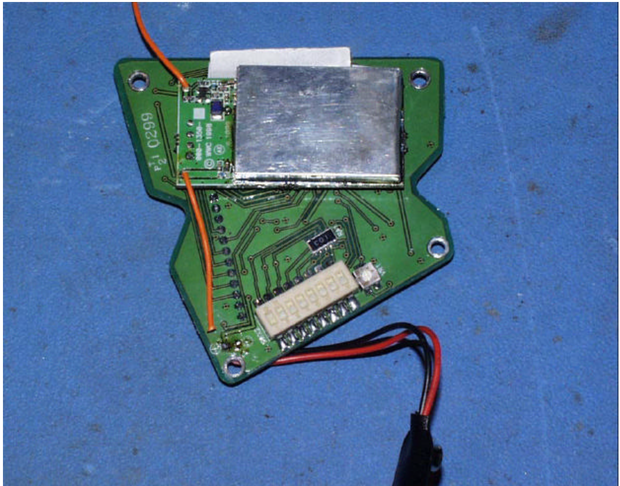
Transceiver and Control Board, Closeup View
