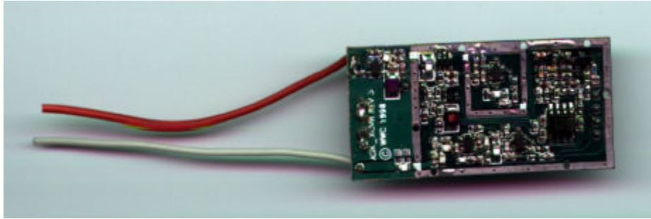
Transceiver Module, Component Side without Shield
