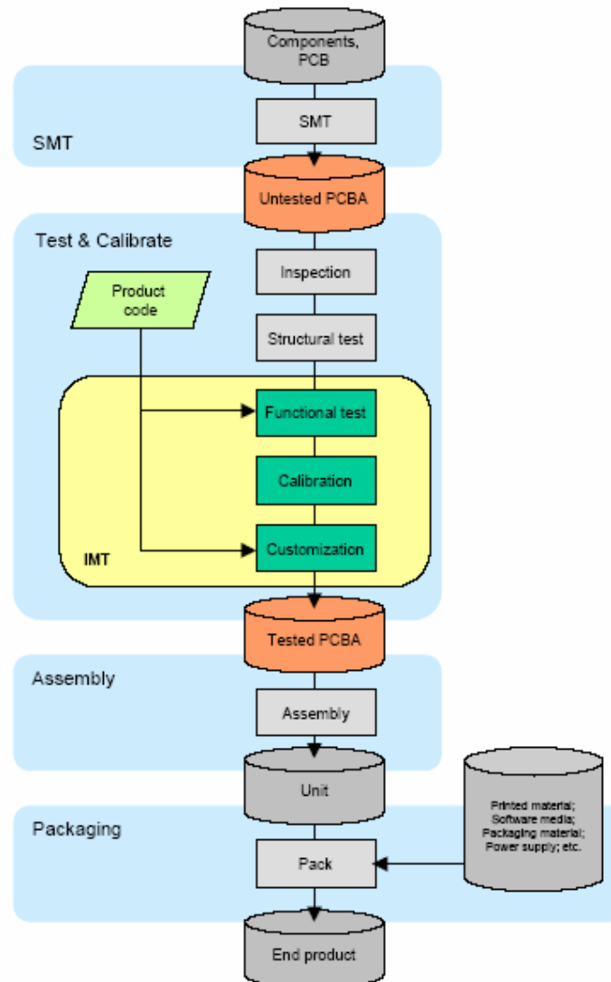
Figure 1. Manufacturing Test Process
