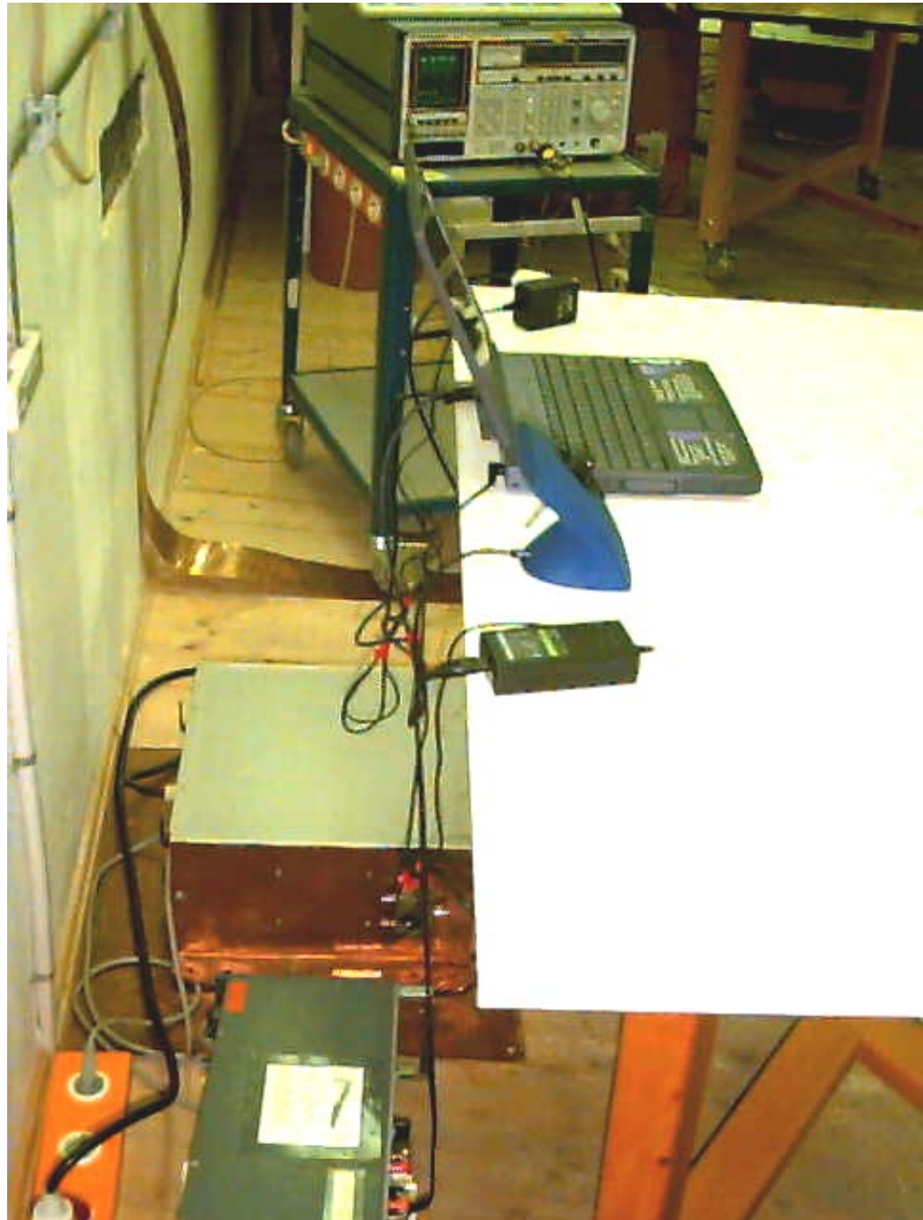
Photograph 1.2: EUT and Peripherals on Non-Conductive Table; Left Side View
