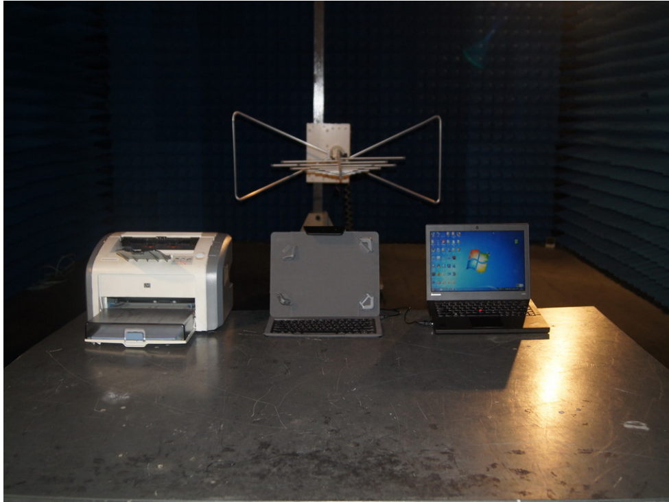
Photograph 8: Set-up for radio spectrum test
