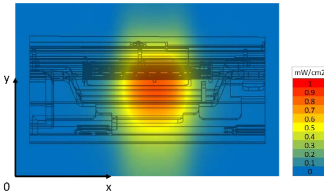
Figure 20 – Channel 3 worst case - Integrated power over 1\text{cm}^2 on a platform
