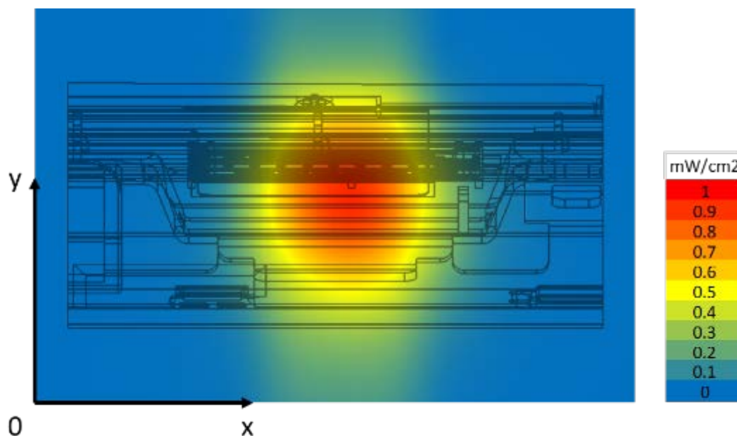
Figure 19 – Channel 2 worst case - Integrated power over 1\text{cm}^2 on a platform
