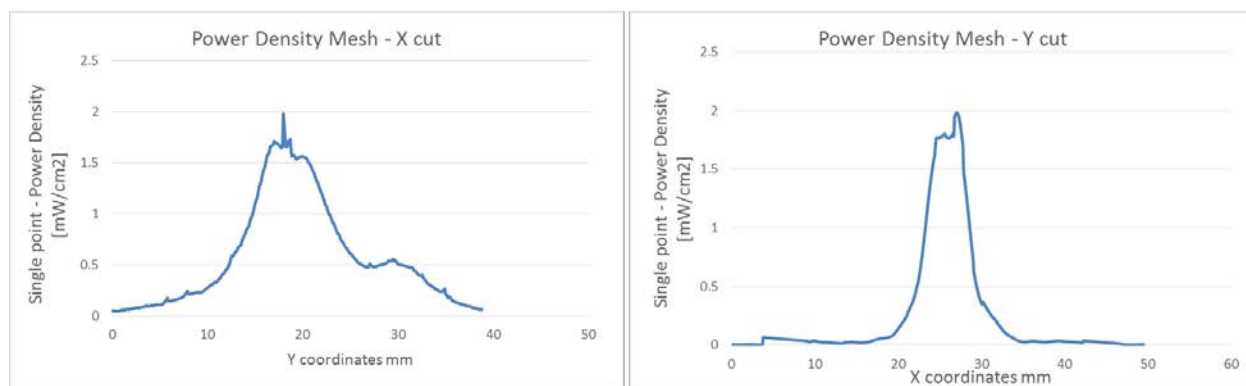
Figure 17 – One dimensional plots of the power density on Channel 3
