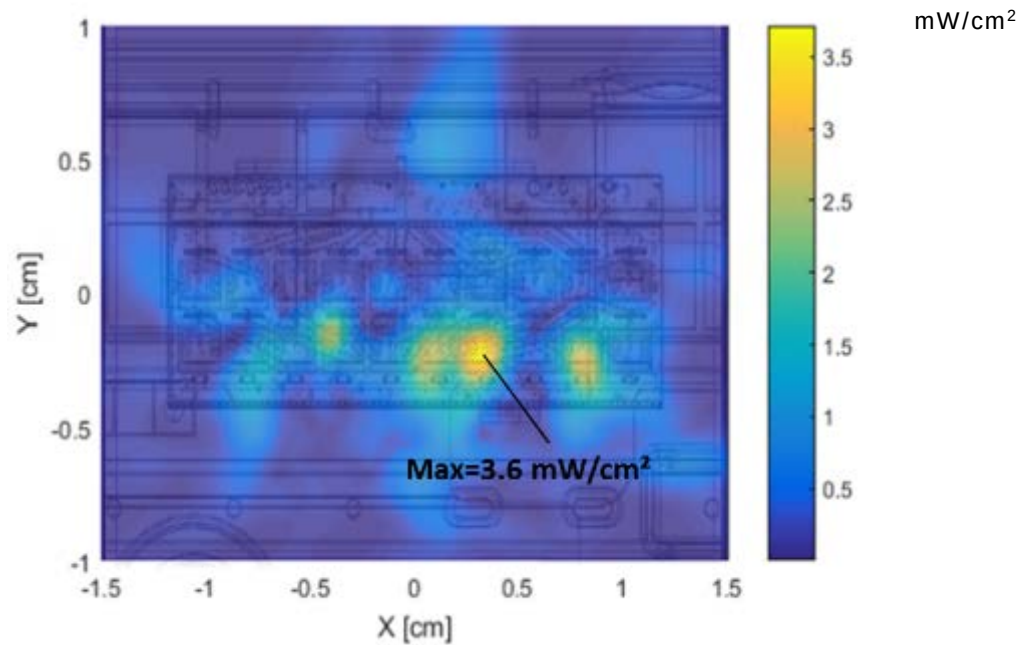
Figure 16 – Channel 3 single-point power density mesh
