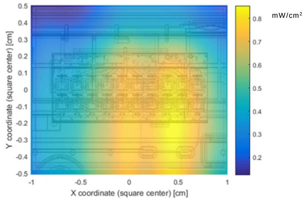
Figure 22 – Channel 3 worst case – integrated power over 1cm 2 and platform
