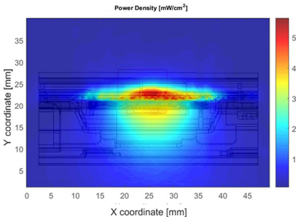
Figure 9 – Channel 2 upper bound, Single-point Power Density
