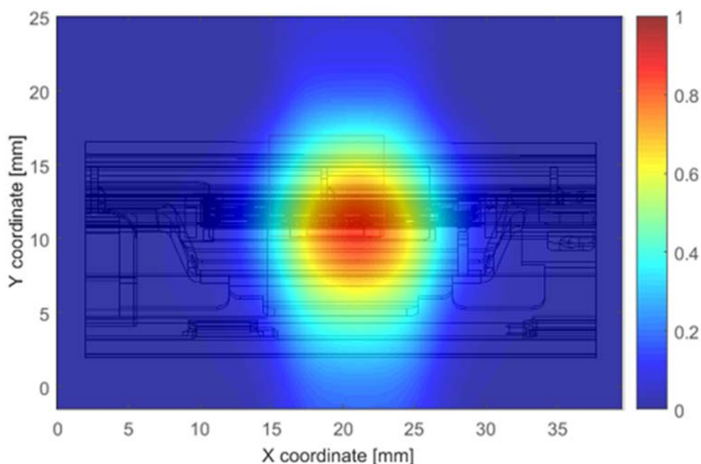
Figure 18 – Channel 1 worst case - Integrated power over 1cm 2 an platform
