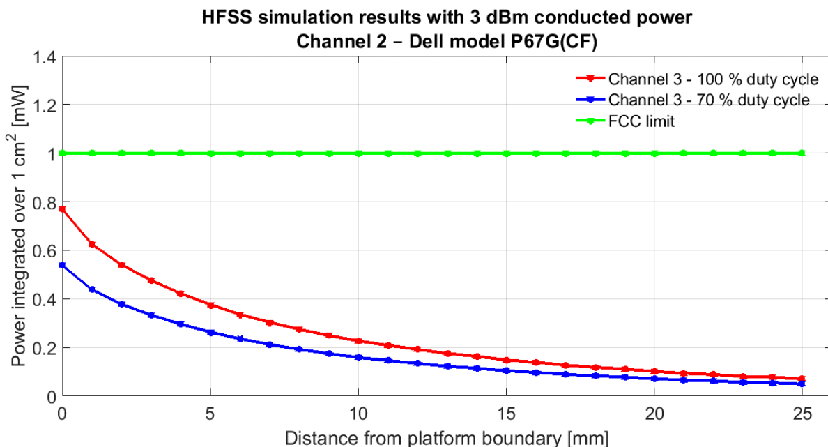
Figure 22 – HFSS Simulation results in Ch2
