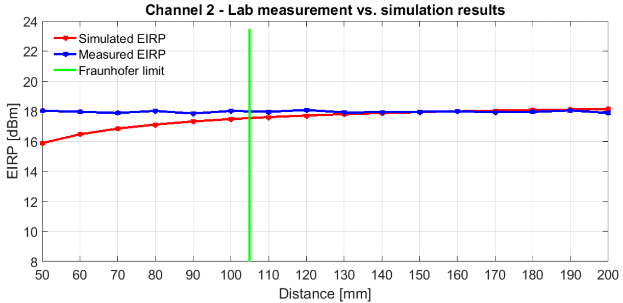
Figure 26 – Comparison of E.I.R.P. simulation to lab measurements – channel 2
