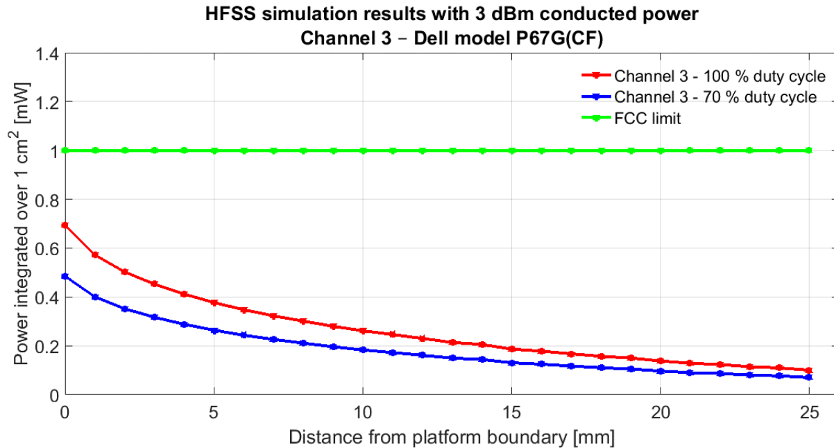
Figure 23 – HFSS Simulation results in Ch3
