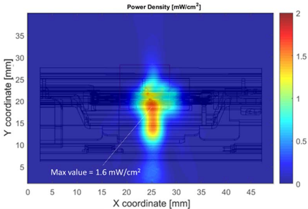
Figure 13 – Channel 2 single-point power density mesh
