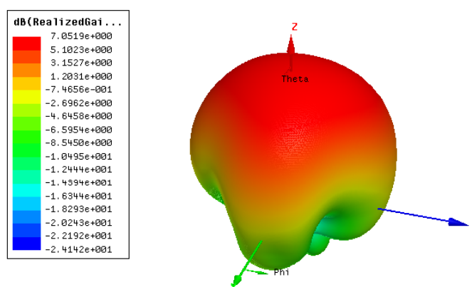
Figure 30 – Patch Antenna Gain
