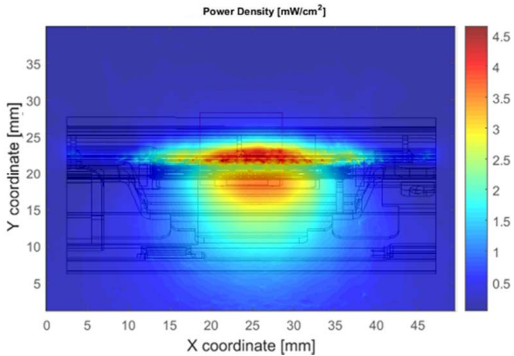
Figure 10 – Channel 3 upper bound, Single-point Power Density mesh
