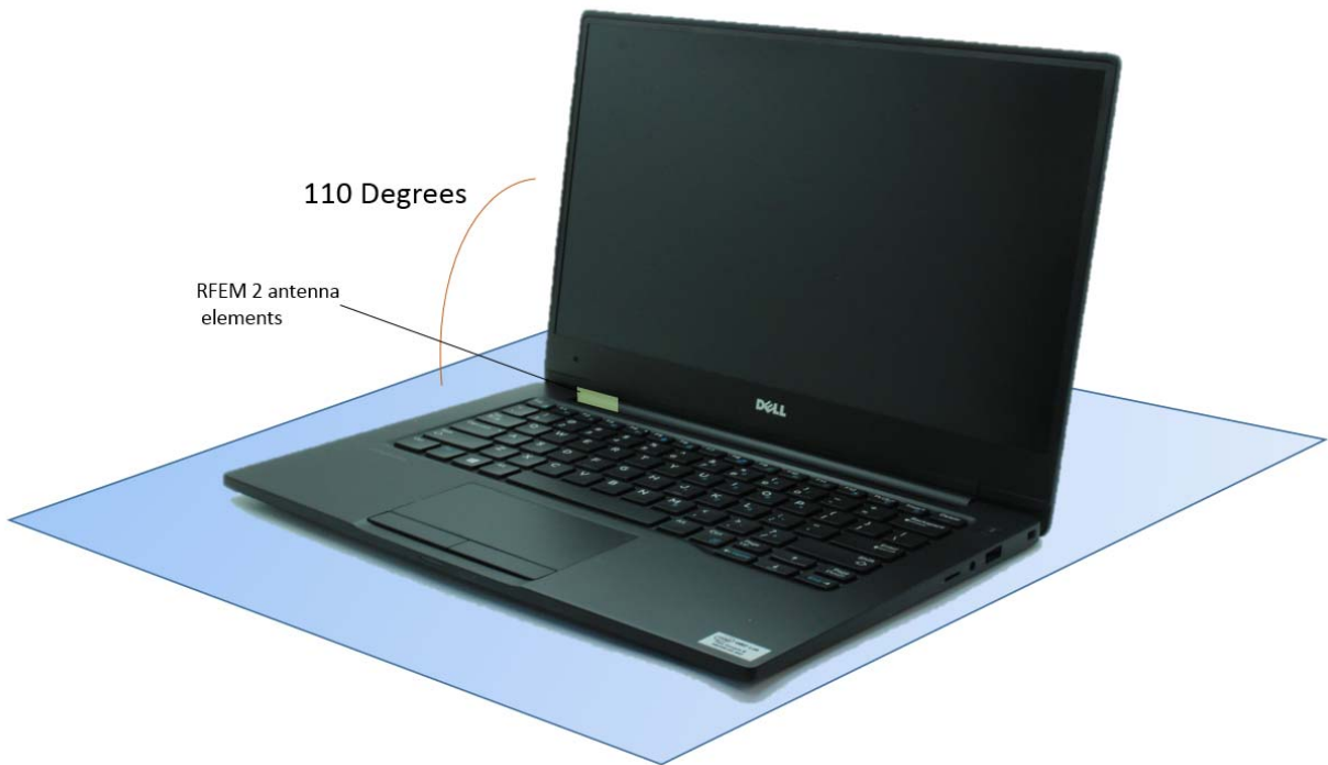
Figure 5 - Platform operating modes
