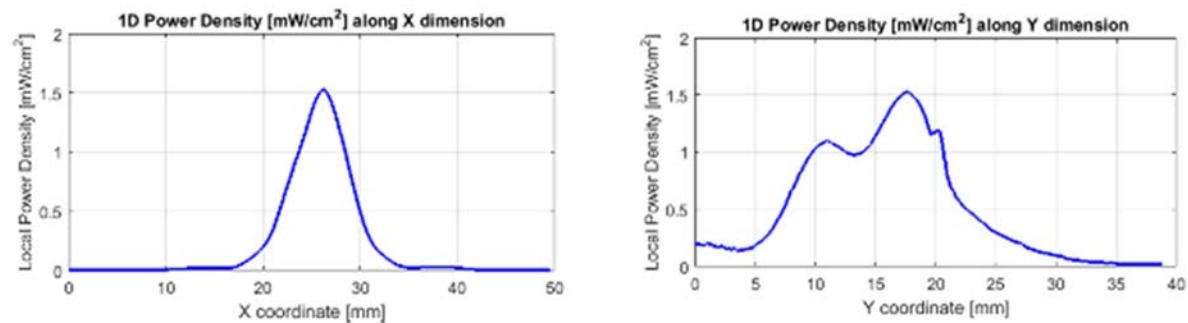
Figure 17 – One dimensional plots of the power density on Channel 3
