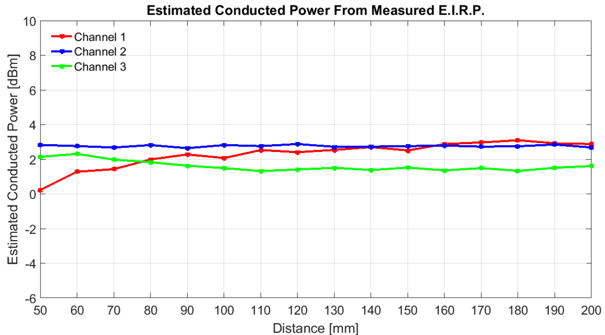
Figure 28 – Estimate conducted power from E.I.R.P. data
