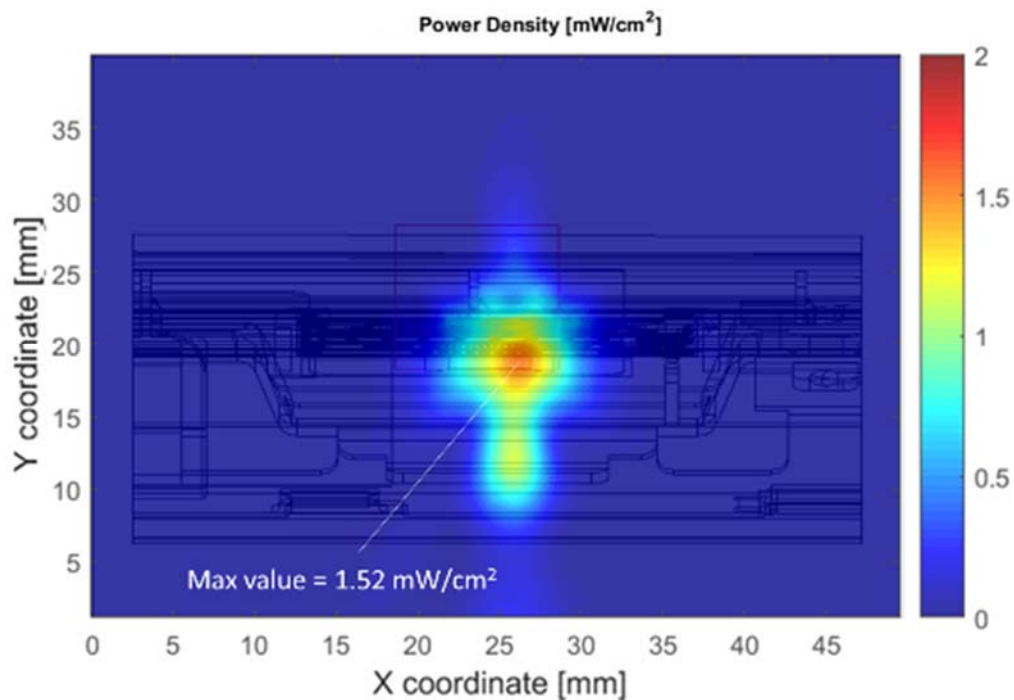
Figure 14 – Channel 3 single-point power density mesh
