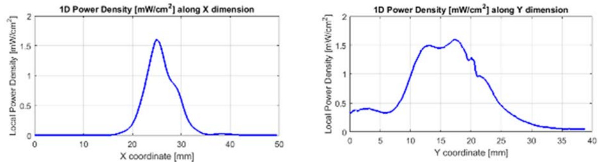
Figure 16 – One dimensional plots of the power density on Channel 2
