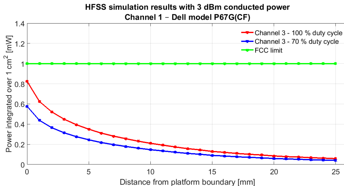
Figure 21 – HFSS Simulation results in Ch1
