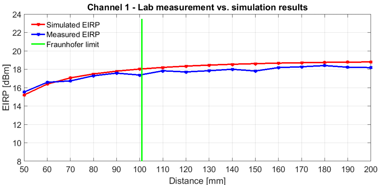
Figure 25 – Comparison of E.I.R.P. simulation to lab measurements – channel 1
