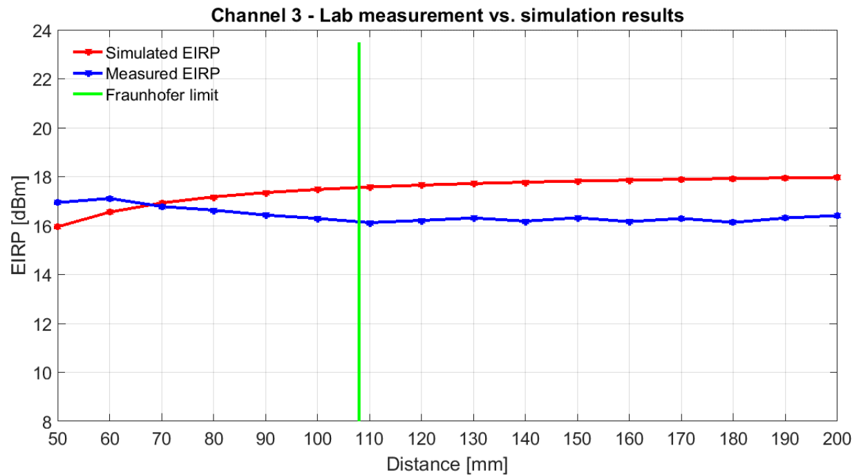
Figure 27 – Comparison of E.I.R.P. simulation to lab measurements – channel 3
