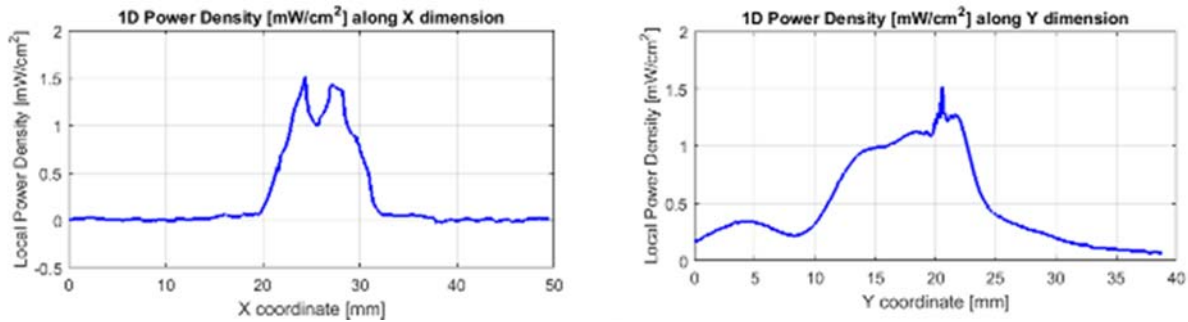
Figure 15 – One dimensional plots of the power density on Channel 1
