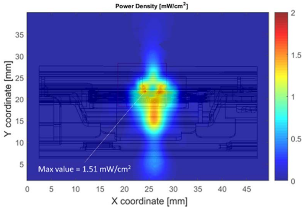
Figure 12 – Channel 1 single-point power density mesh
