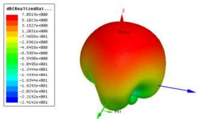
Figure 51 – Patch Antenna Gain
