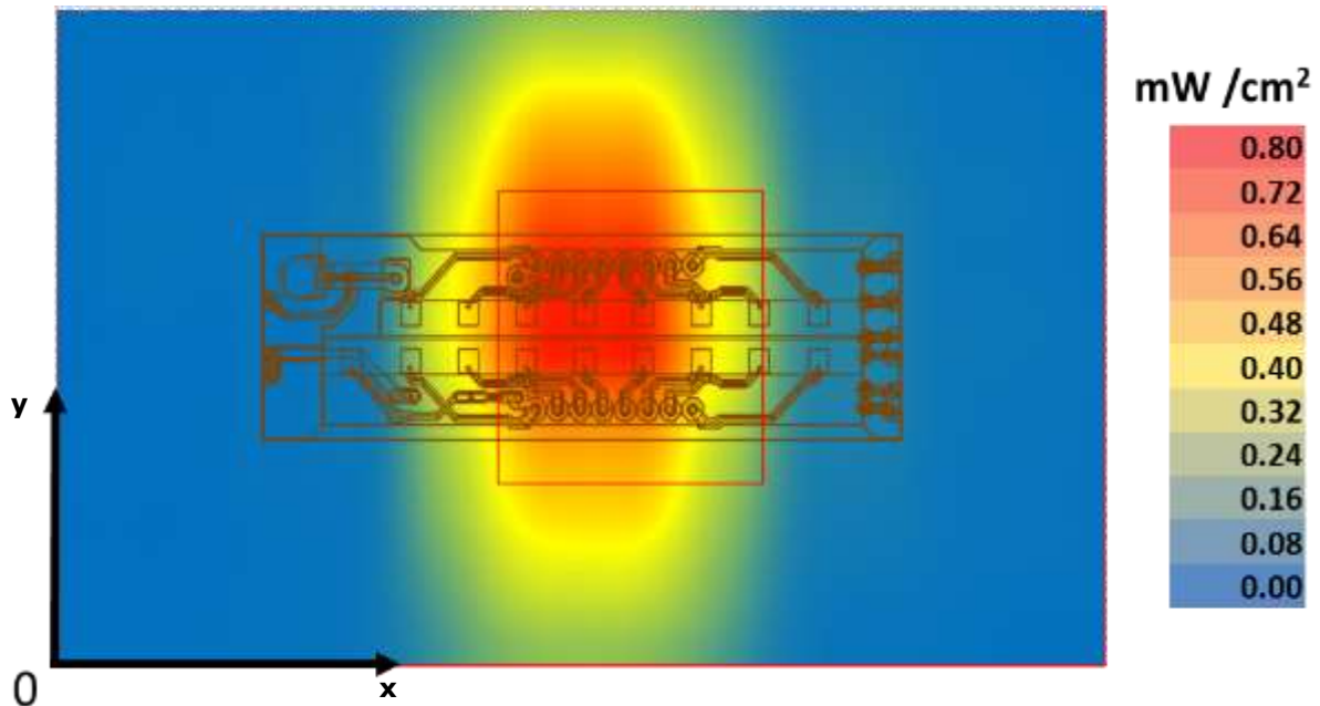
Figure 40 – Channel 2 worst case - Integrated power over 1cm² on platform base
