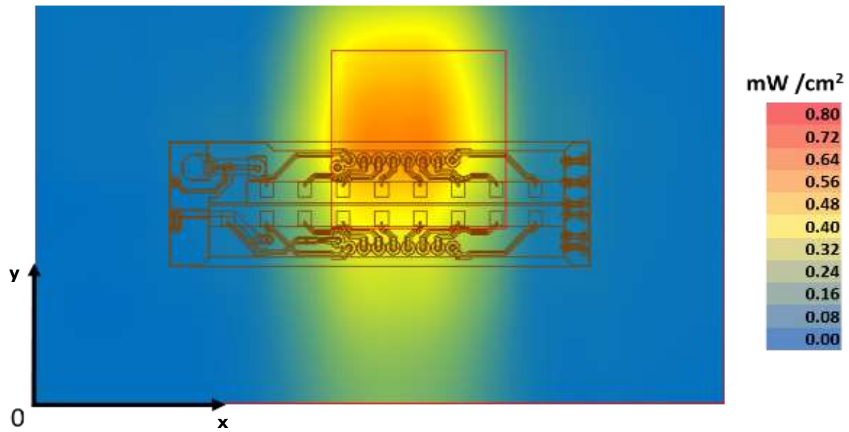
Figure 41 – Channel 3 Worst case - Integrated power over 1cm 2 on platform base
