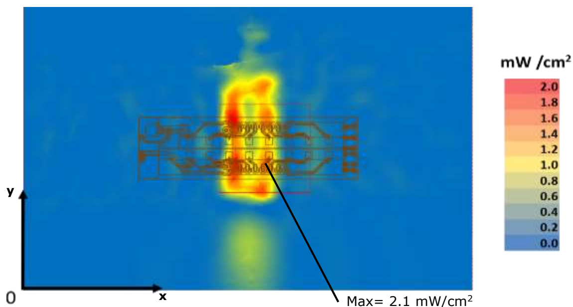
Figure 34 – Channel 2 single-point power density mesh on platform base
