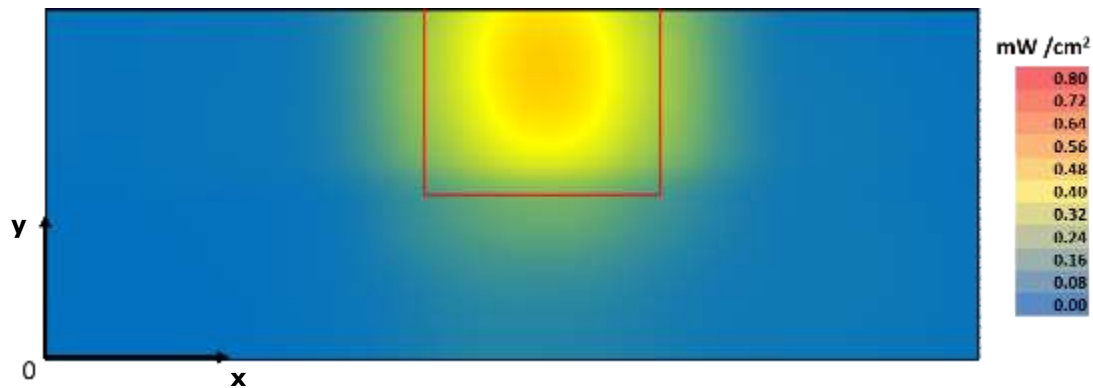
Figure 23 – Channel 3 worst case - Integrated power over 1\text{cm}^2 on platform edge
