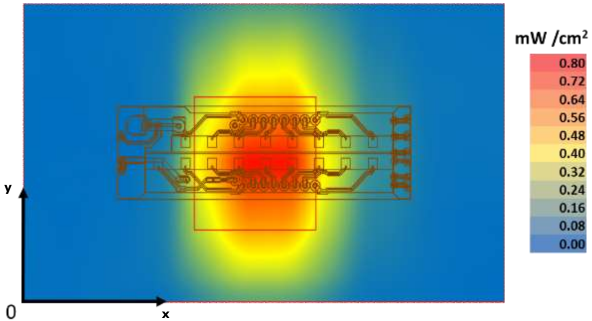
Figure 39 – Channel 1 worst case - Integrated power over 1cm² on platform base
