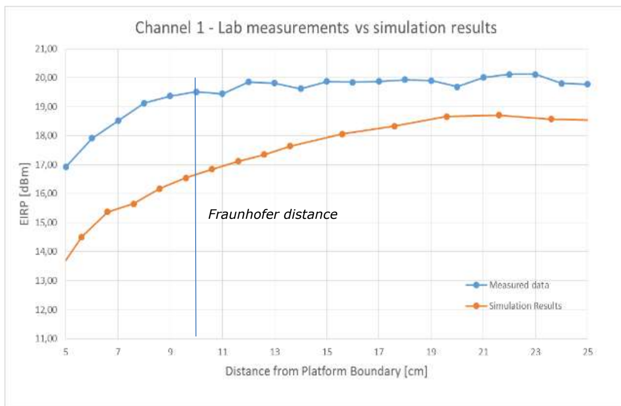
Figure 46 – Comparison of E.I.R.P. simulation to lab measurements – channel 1
