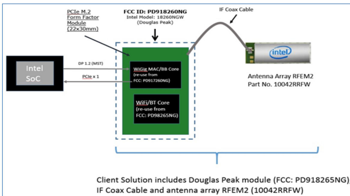
Figure 1 – Intel 18260NGW module system block diagram
