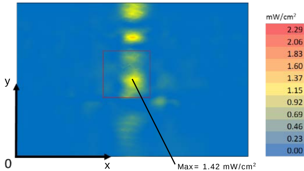
Figure 16 – Channel 2 single-point power density mesh on platform edge
