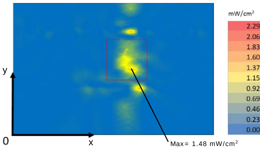
Figure 17 – Channel 3 single-point power density mesh on platform edge
