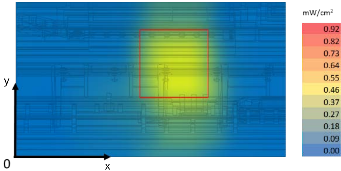
Figure 23 – Channel 3 worst case - Integrated power over 1\text{cm}^2 on platform edge
