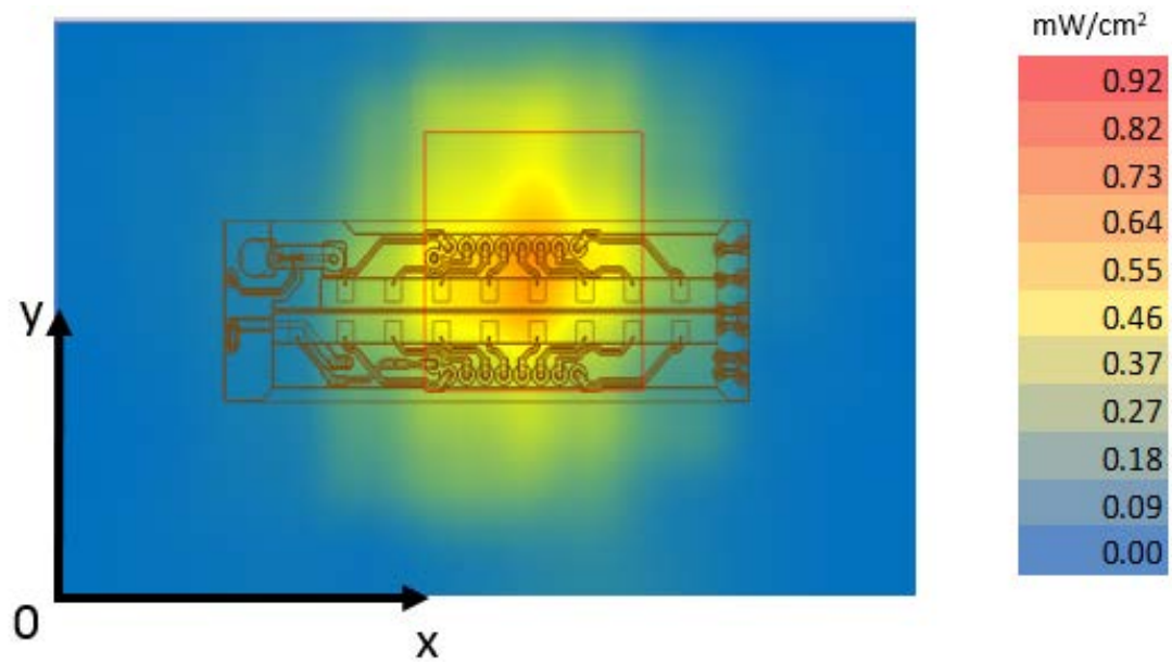
Figure 35 – Channel 2 worst case - Integrated power over 1cm 2 on platform base
