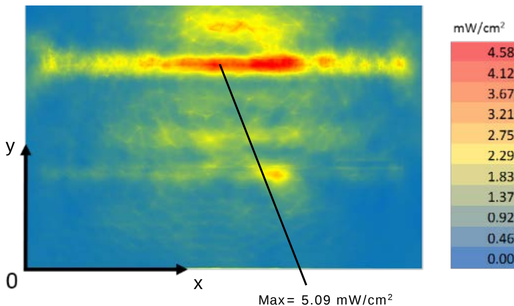
Figure 12 – Channel 2 upper bound, Single-point power density mesh on platform edge at 100 % duty cycle
