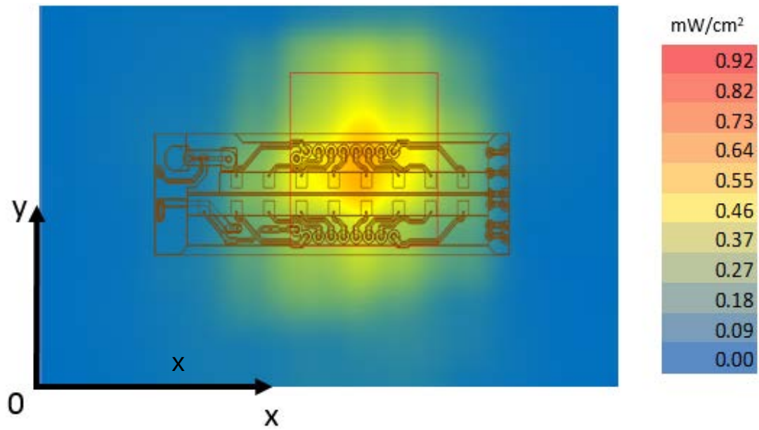
Figure 36 – Channel 3 worst case - Integrated power over 1cm 2 an platform edge
