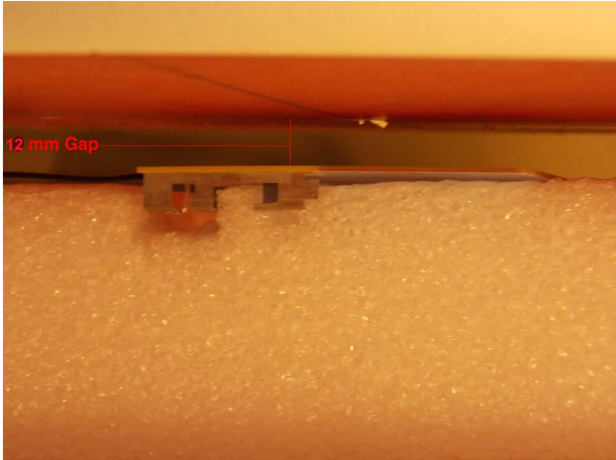
Test Position Side A 12 mm Gap
