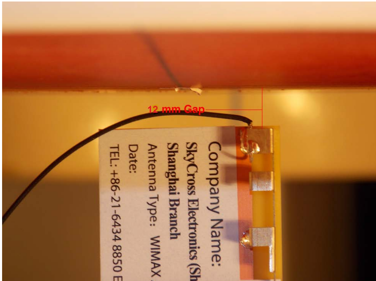
Test Position Side C 12 mm Gap
