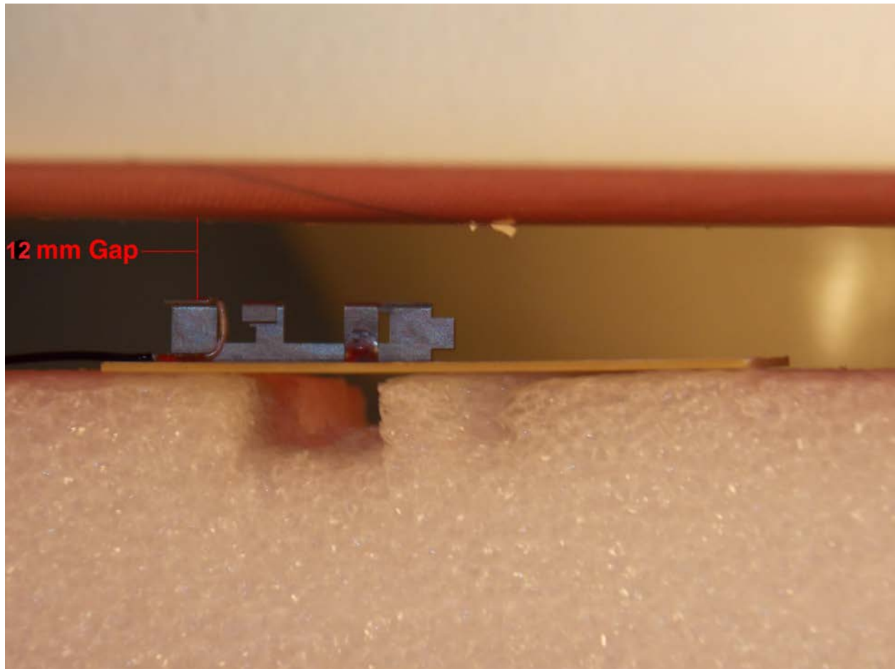
Test Position Side B 12 mm Gap
