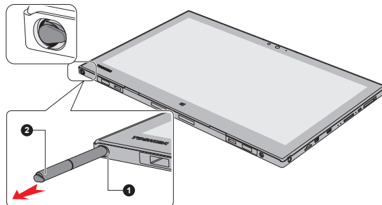
Figure 4-9 Removing the Reserve Pen
