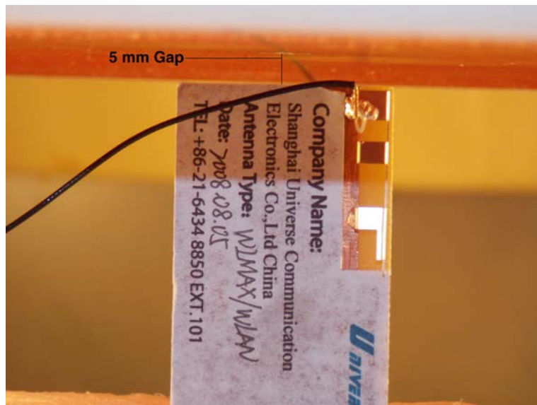
Test Position Side C 5 mm Gap
