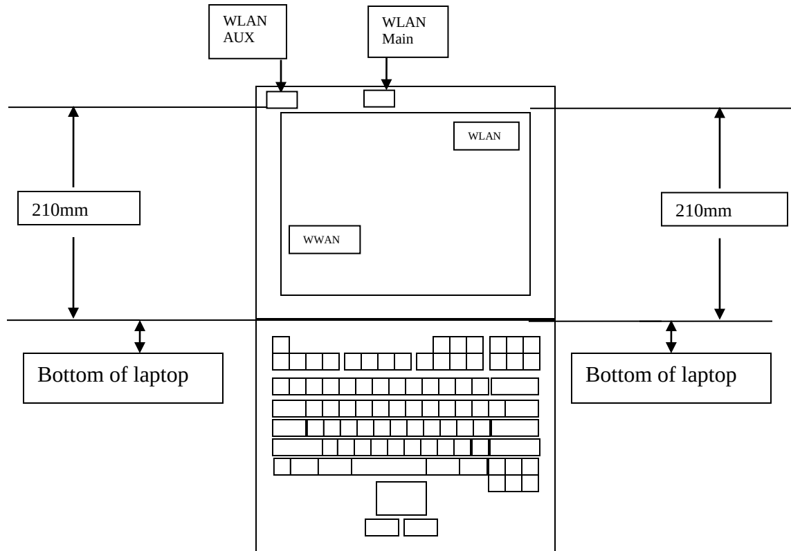
Module and Antenna Locations
