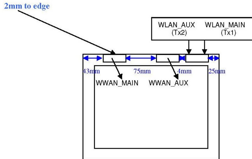
Module and Antenna Locations 13.5"
