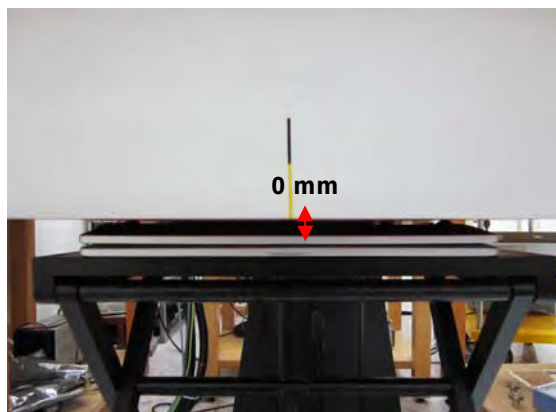
Fig.3 EUT Lap-held mode to flat phantom
