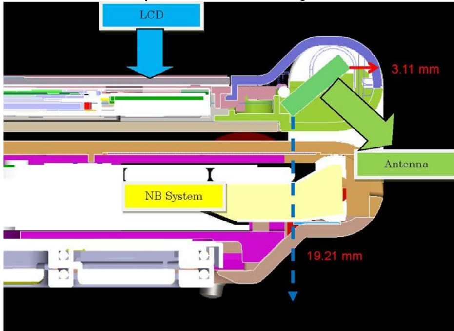
Location and Separation Distances Diagrams Tablet Mode
