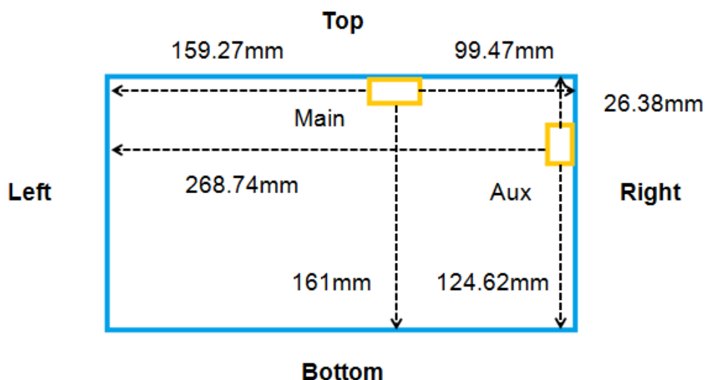
Front view of the tablet
