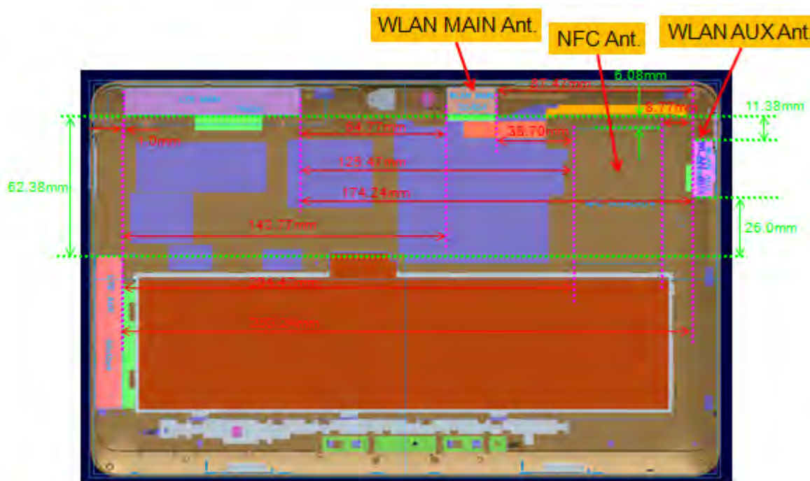
Fig.8 Antenna position of EUT
