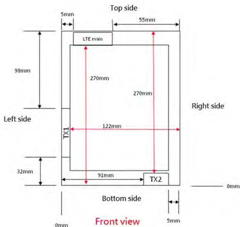
Fig.10 Antenna position of EUT (Front view)
