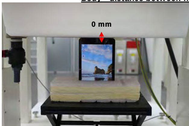
Fig.3 EUT Top side to flat phantom
