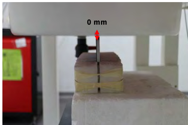
Fig.6 EUT Right side to flat phantom
