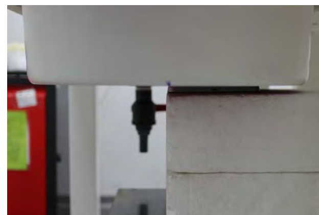
Fig.4 EUT Back side to flat phantom
