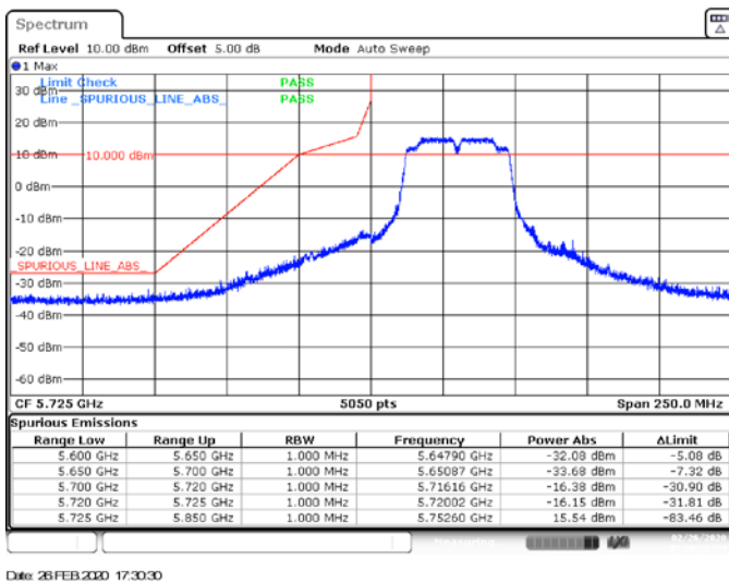
MIMO A, 802.11n40, HT8, CH151, BE Low Peak
