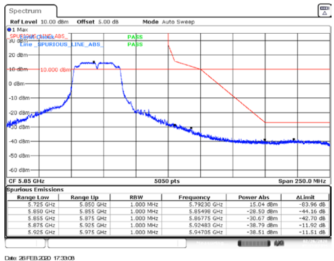
MIMO A, 802.11n40, HT8, CH159, BE High Peak
