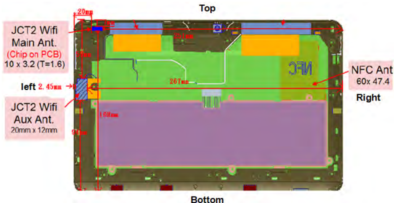
Fig.8 Antenna position of EUT (Front view)
