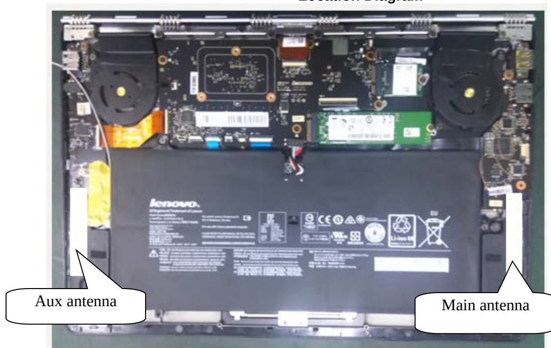
Location Diagram
