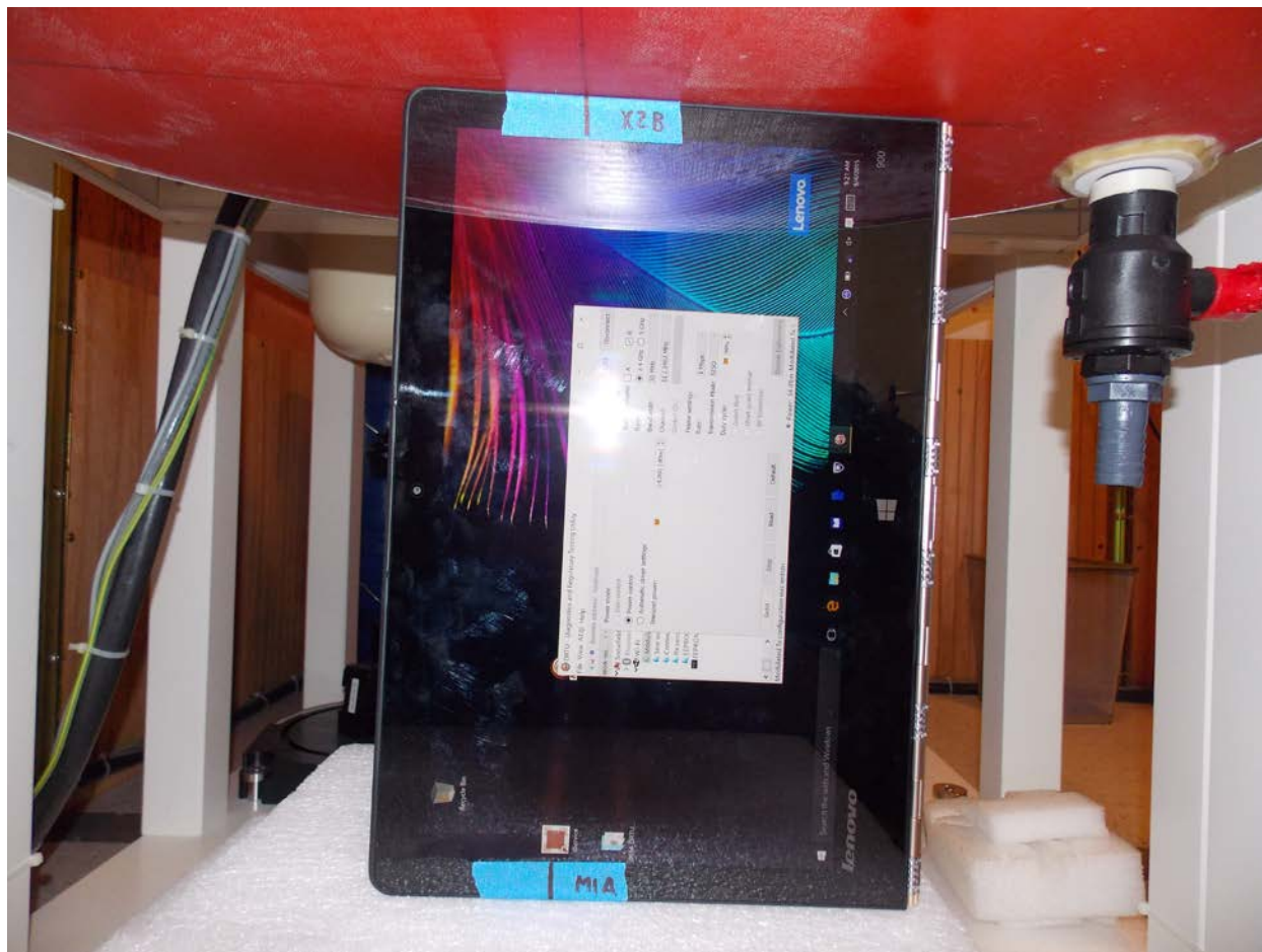
Test Position Tablet Right 0 mm Gap
